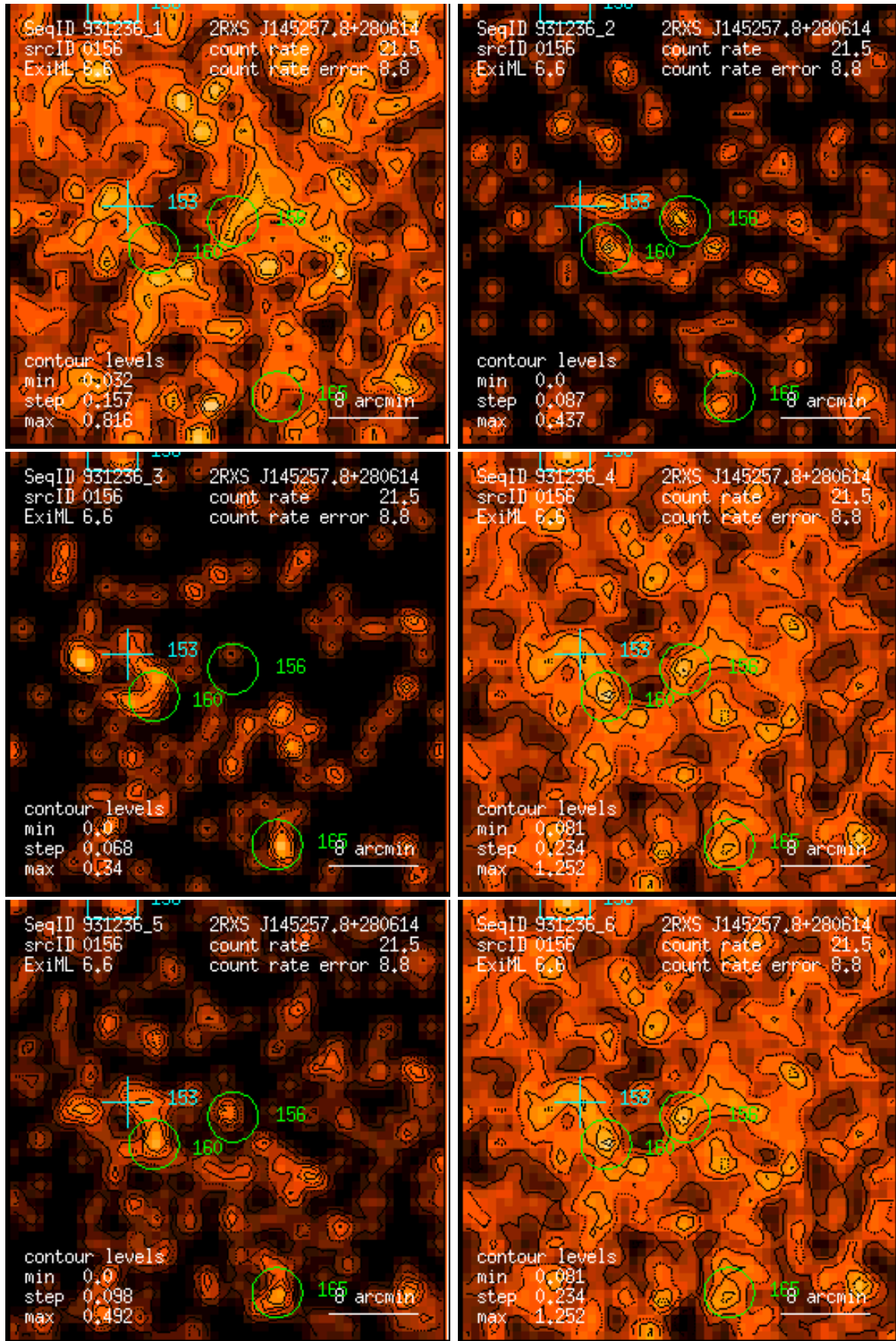
Figure 156: RASS 931236: detection 0156: band rate images, Gaussian filter: (1) PSPC channels 11 – 41, (2) 52 – 90, (3) 91 – 201, (4) 11 – 235, (5) 52 – 201, (6) 11 – 201. Broad band rates in counts/ks. Band rate contour levels in counts/ks/arcmin 2 .
