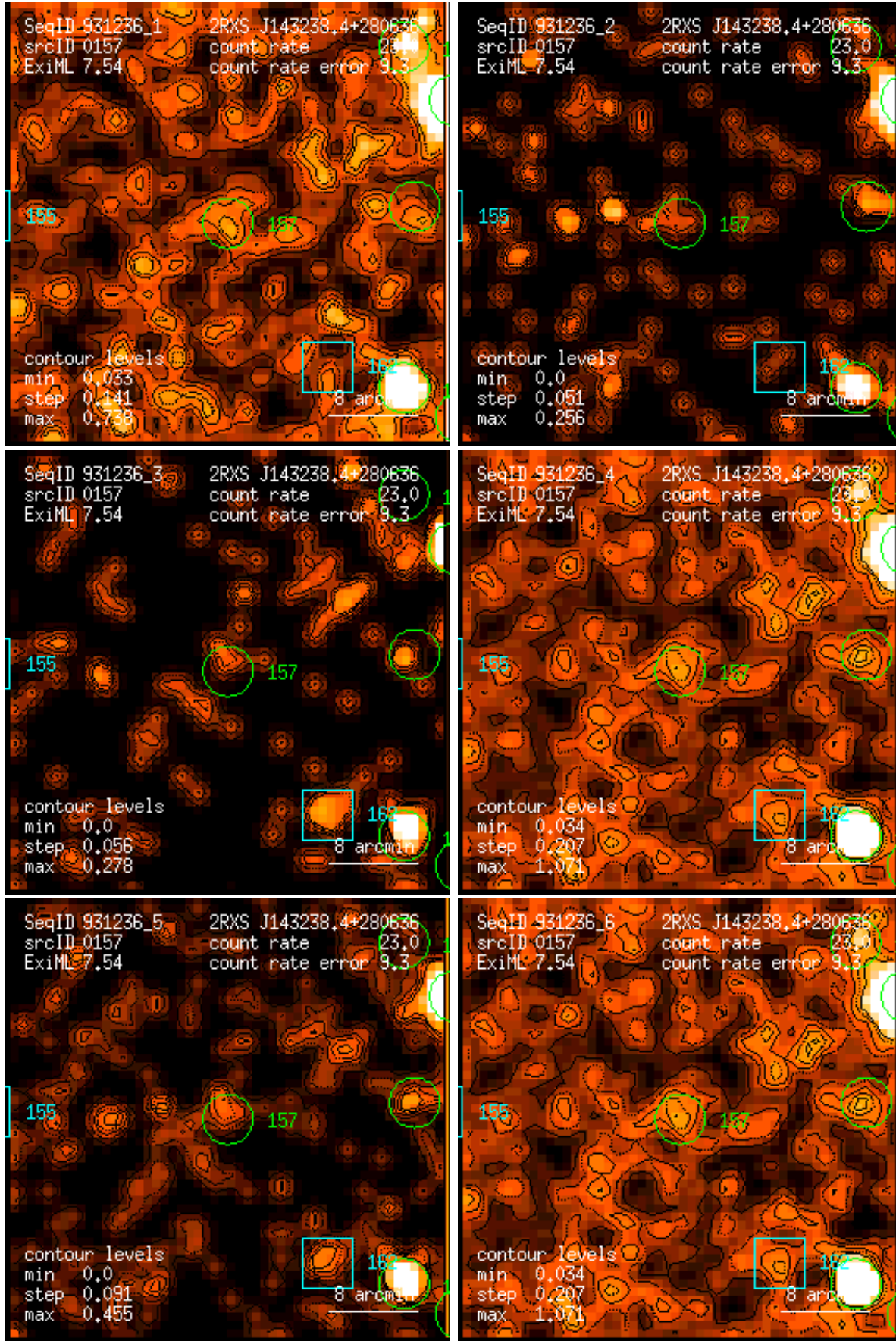
Figure 157: RASS 931236: detection 0157: band rate images, Gaussian filter: (1) PSPC channels 11 – 41, (2) 52 – 90, (3) 91 – 201, (4) 11 – 235, (5) 52 – 201, (6) 11 – 201. Broad band rates in counts/ks. Band rate contour levels in counts/ks/arcmin 2 .
