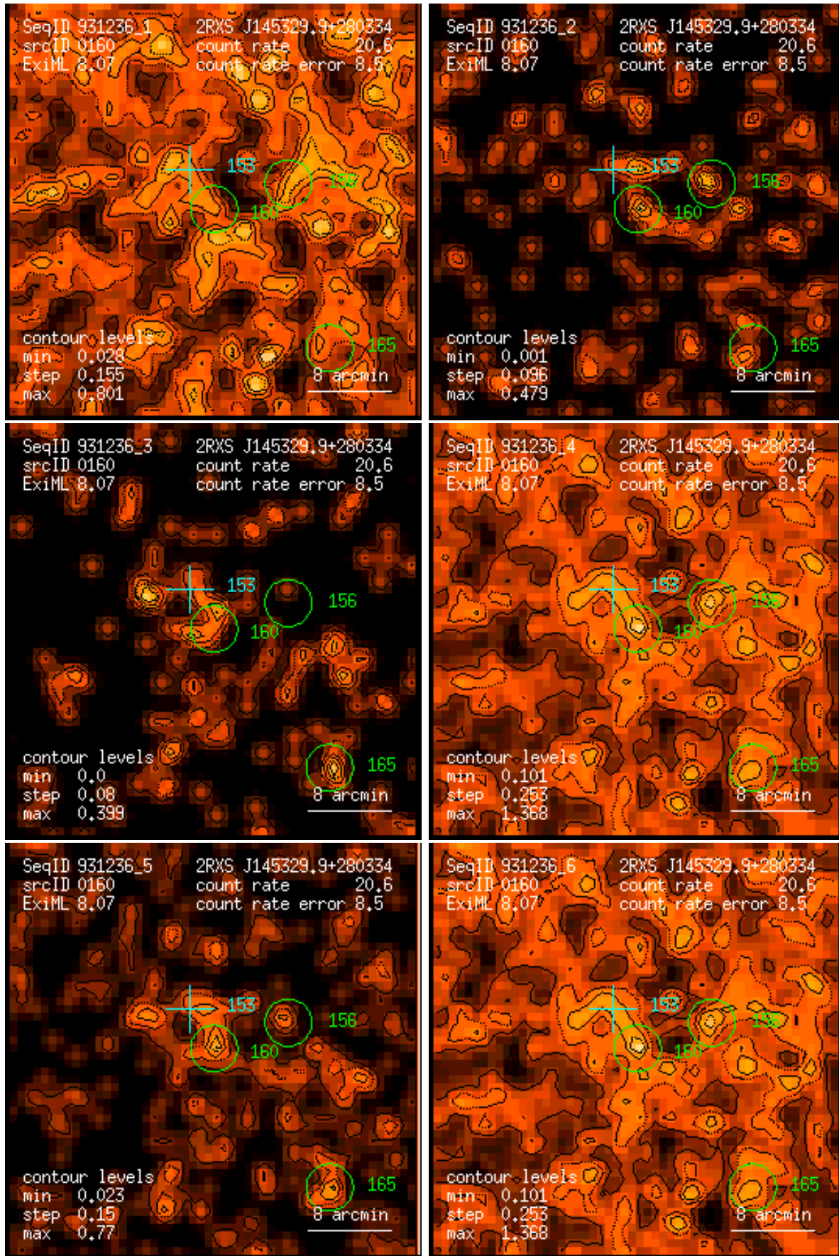
Figure 160: RASS 931236: detection 0160: band rate images, Gaussian filter: (1) PSPC channels 11 – 41, (2) 52 – 90, (3) 91 – 201, (4) 11 – 235, (5) 52 – 201, (6) 11 – 201. Broad band rates in counts/ks. Band rate contour levels in counts/ks/arcmin 2 .
