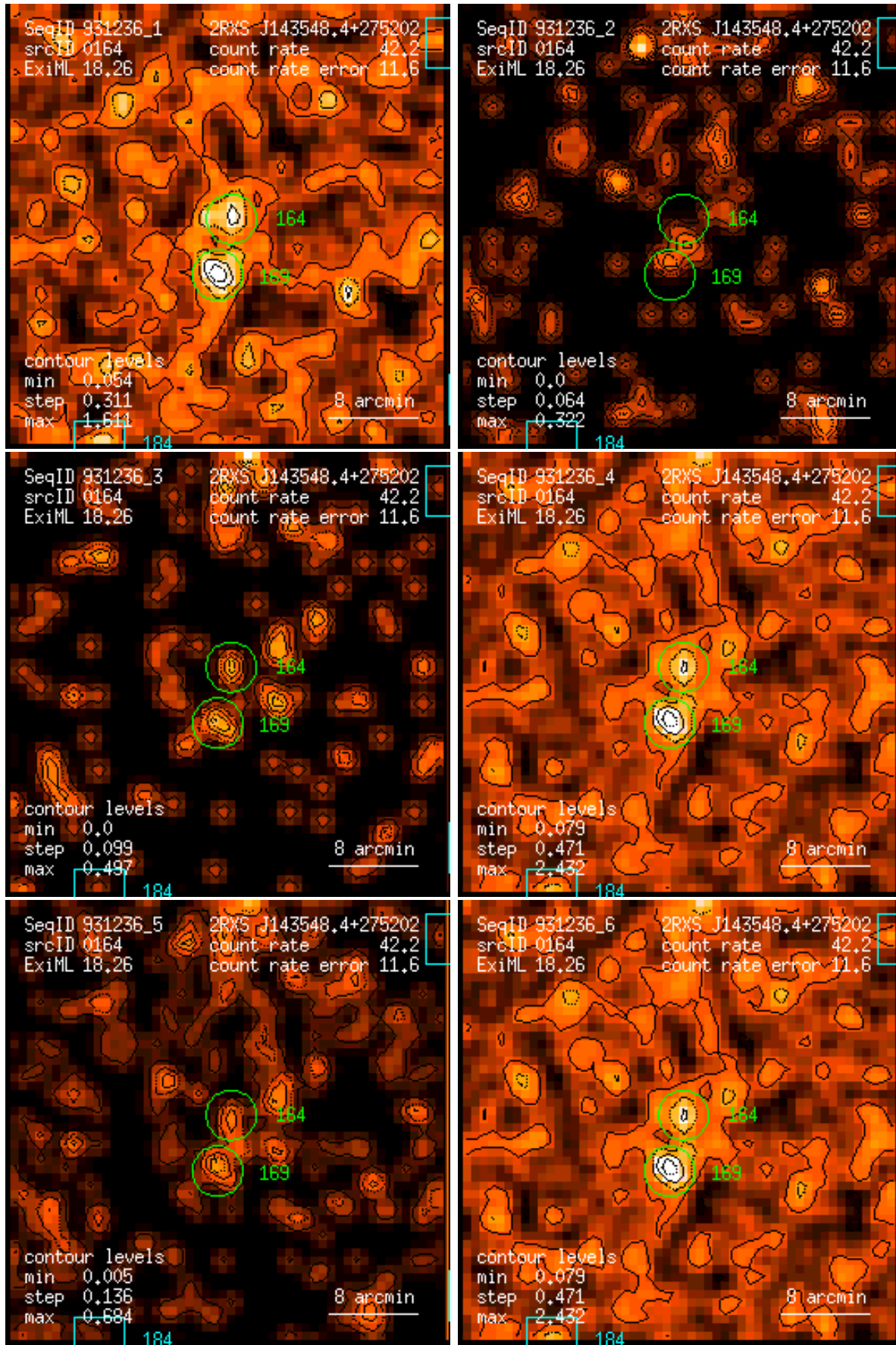
Figure 164: RASS 931236: detection 0164: band rate images, Gaussian filter: (1) PSPC channels 11 – 41, (2) 52 – 90, (3) 91 – 201, (4) 11 – 235, (5) 52 – 201, (6) 11 – 201. Broad band rates in counts/ks. Band rate contour levels in counts/ks/arcmin 2 .
