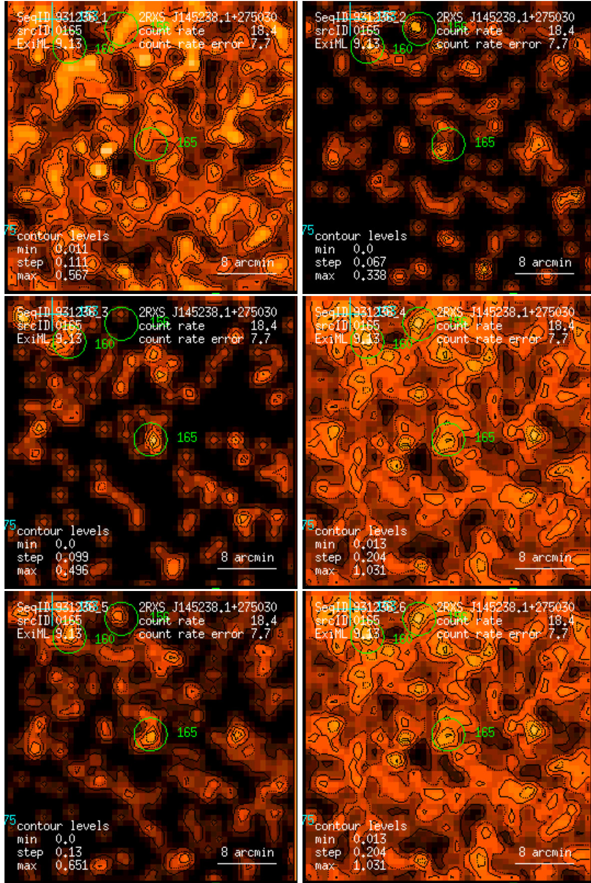
Figure 165: RASS 931236: detection 0165: band rate images, Gaussian filter: (1) PSPC channels 11 – 41, (2) 52 – 90, (3) 91 – 201, (4) 11 – 235, (5) 52 – 201, (6) 11 – 201. Broad band rates in counts/ks. Band rate contour levels in counts/ks/arcmin 2 .
