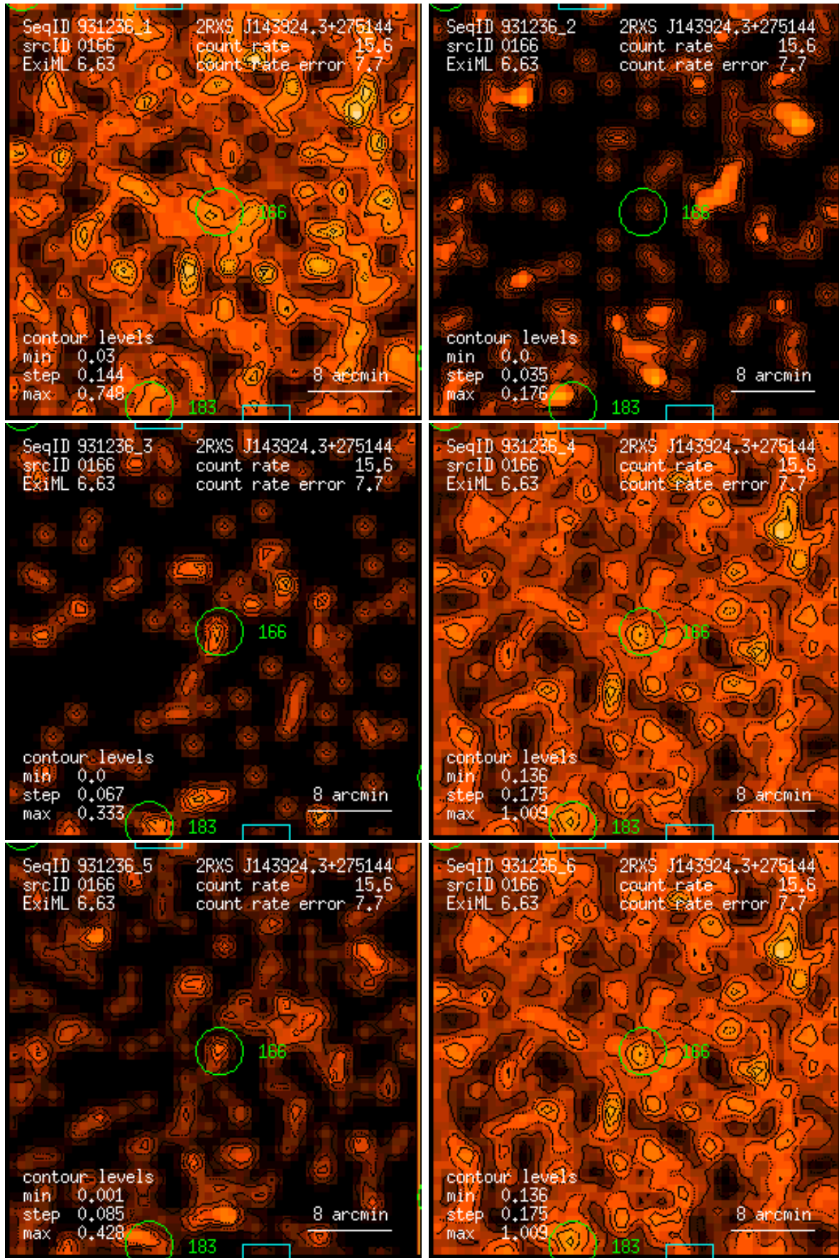
Figure 166: RASS 931236: detection 0166: band rate images, Gaussian filter: (1) PSPC channels 11 – 41, (2) 52 – 90, (3) 91 – 201, (4) 11 – 235, (5) 52 – 201, (6) 11 – 201. Broad band rates in counts/ks. Band rate contour levels in counts/ks/arcmin 2 .
