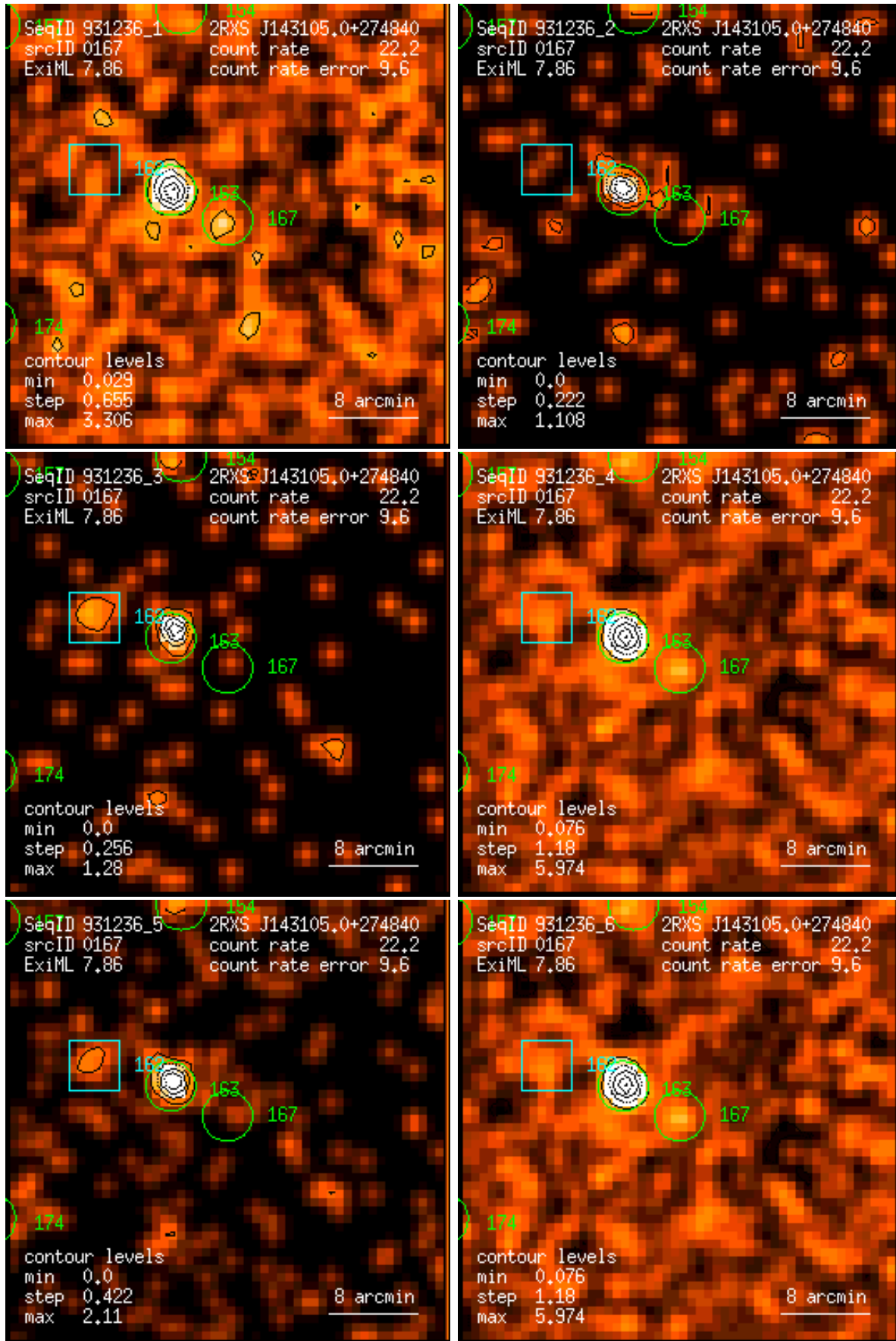
Figure 167: RASS 931236: detection 0167: band rate images, Gaussian filter: (1) PSPC channels 11 – 41, (2) 52 – 90, (3) 91 – 201, (4) 11 – 235, (5) 52 – 201, (6) 11 – 201. Broad band rates in counts/ks. Band rate contour levels in counts/ks/arcmin 2 .
