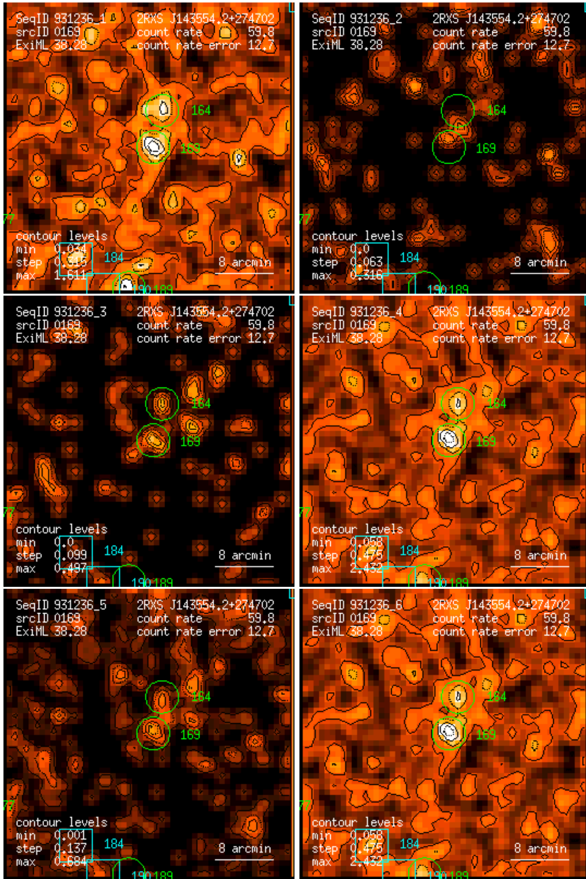
Figure 169: RASS 931236: detection 0169: band rate images, Gaussian filter: (1) PSPC channels 11 – 41, (2) 52 – 90, (3) 91 – 201, (4) 11 – 235, (5) 52 – 201, (6) 11 – 201. Broad band rates in counts/ks. Band rate contour levels in counts/ks/arcmin 2 .
