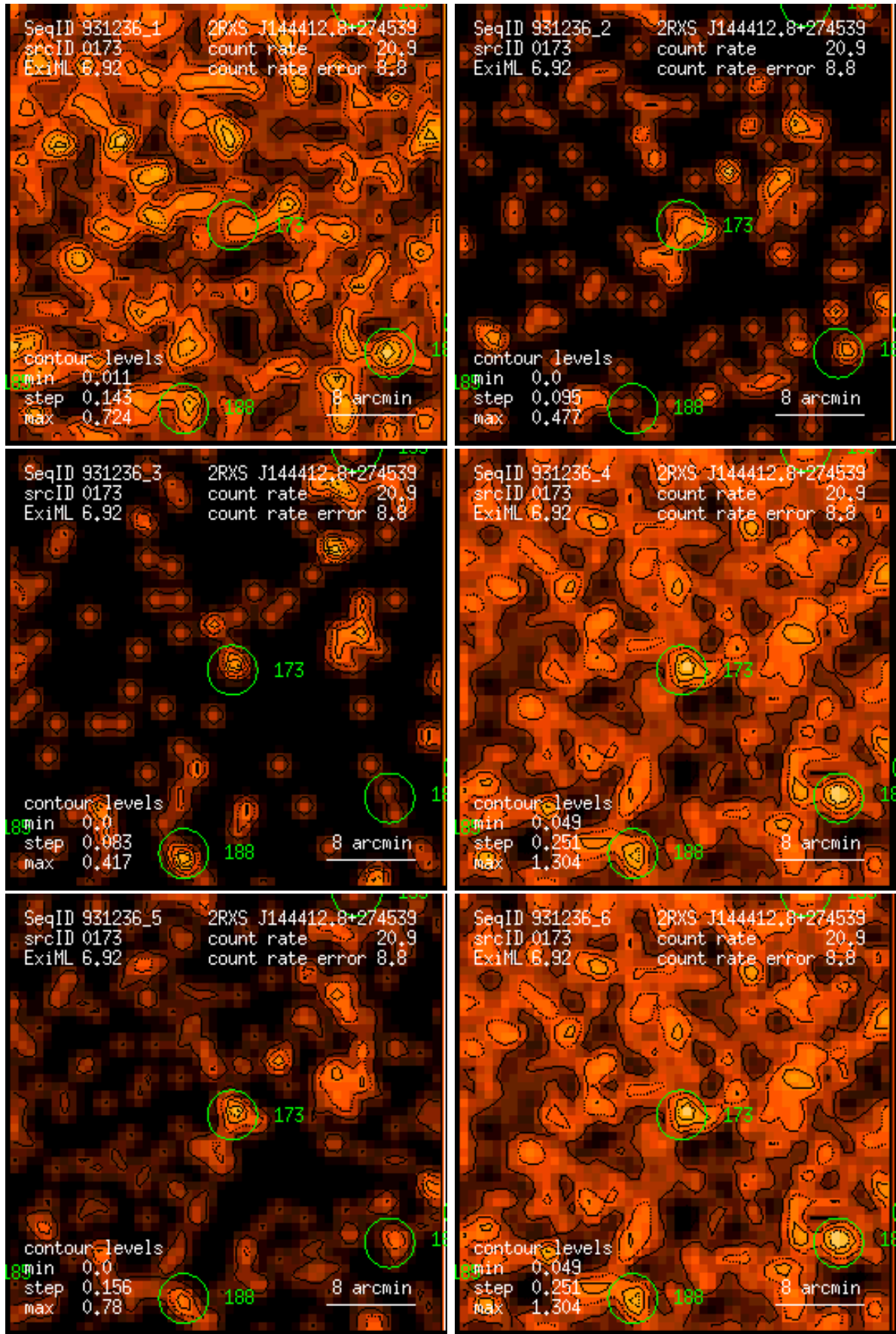
Figure 173: RASS 931236: detection 0173: band rate images, Gaussian filter: (1) PSPC channels 11 – 41, (2) 52 – 90, (3) 91 – 201, (4) 11 – 235, (5) 52 – 201, (6) 11 – 201. Broad band rates in counts/ks. Band rate contour levels in counts/ks/arcmin 2 .
