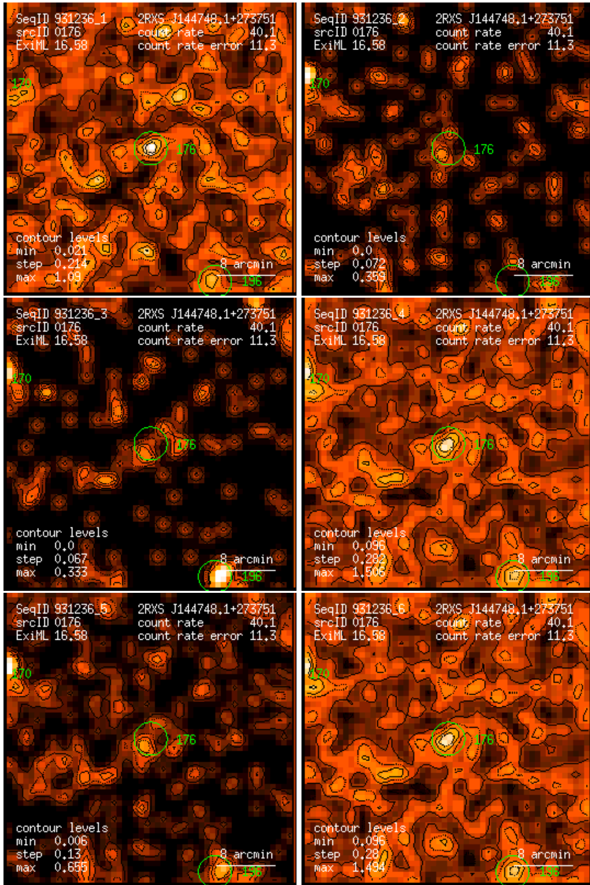
Figure 176: RASS 931236: detection 0176: band rate images, Gaussian filter: (1) PSPC channels 11 – 41, (2) 52 – 90, (3) 91 – 201, (4) 11 – 235, (5) 52 – 201, (6) 11 – 201. Broad band rates in counts/ks. Band rate contour levels in counts/ks/arcmin 2 .
