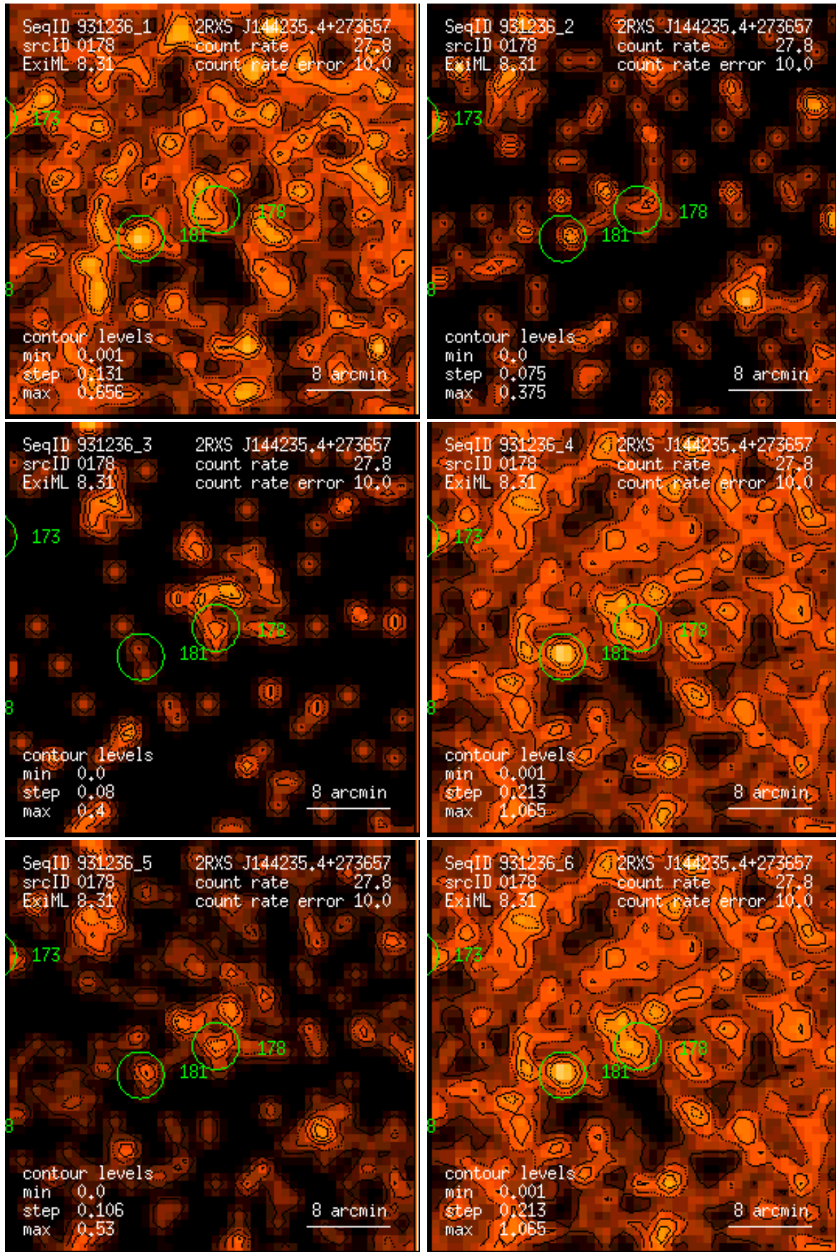
Figure 178: RASS 931236: detection 0178: band rate images, Gaussian filter: (1) PSPC channels 11 – 41, (2) 52 – 90, (3) 91 – 201, (4) 11 – 235, (5) 52 – 201, (6) 11 – 201. Broad band rates in counts/ks. Band rate contour levels in counts/ks/arcmin 2 .
