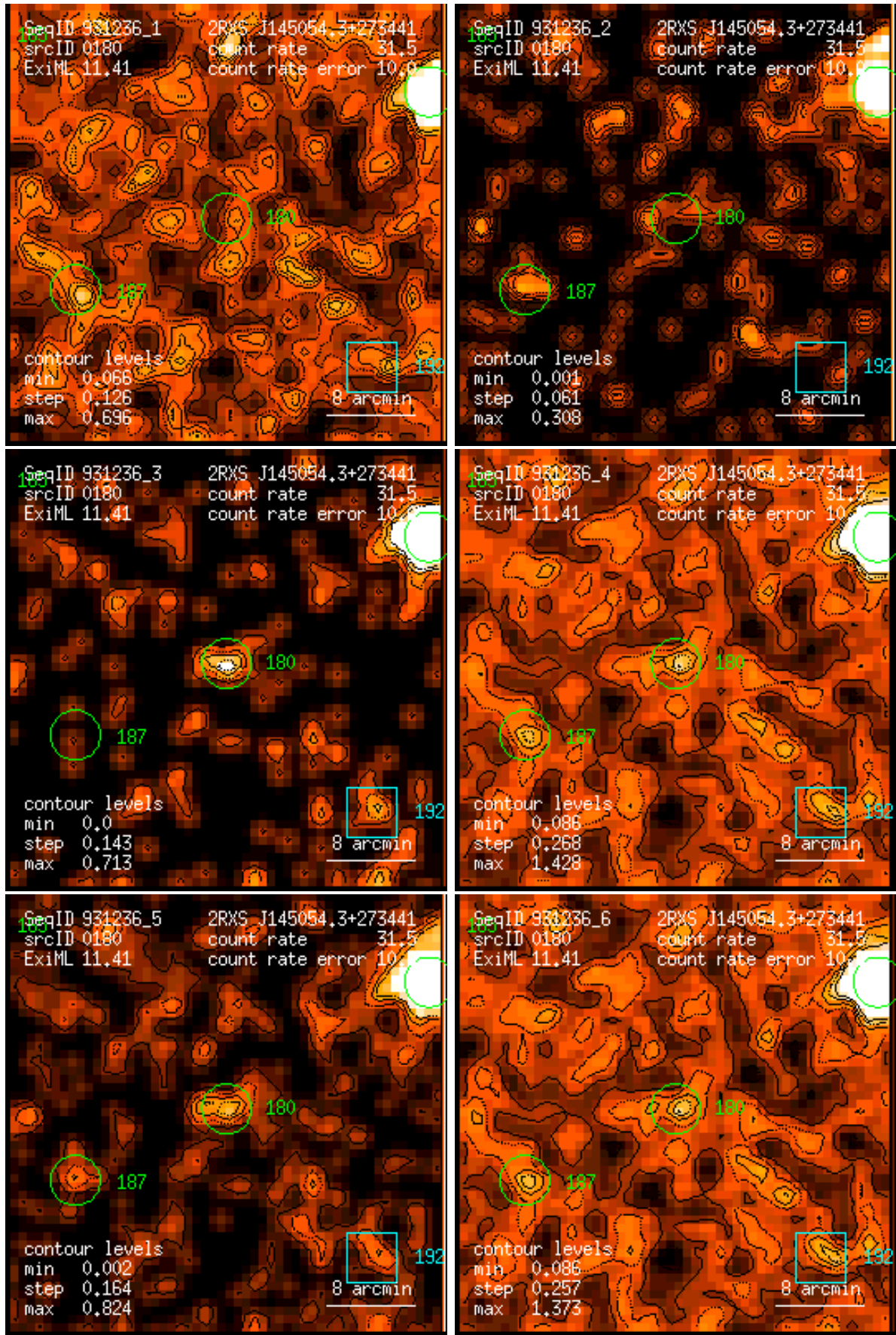
Figure 180: RASS 931236: detection 0180: band rate images, Gaussian filter: (1) PSPC channels 11 – 41, (2) 52 – 90, (3) 91 – 201, (4) 11 – 235, (5) 52 – 201, (6) 11 – 201. Broad band rates in counts/ks. Band rate contour levels in counts/ks/arcmin 2 .
