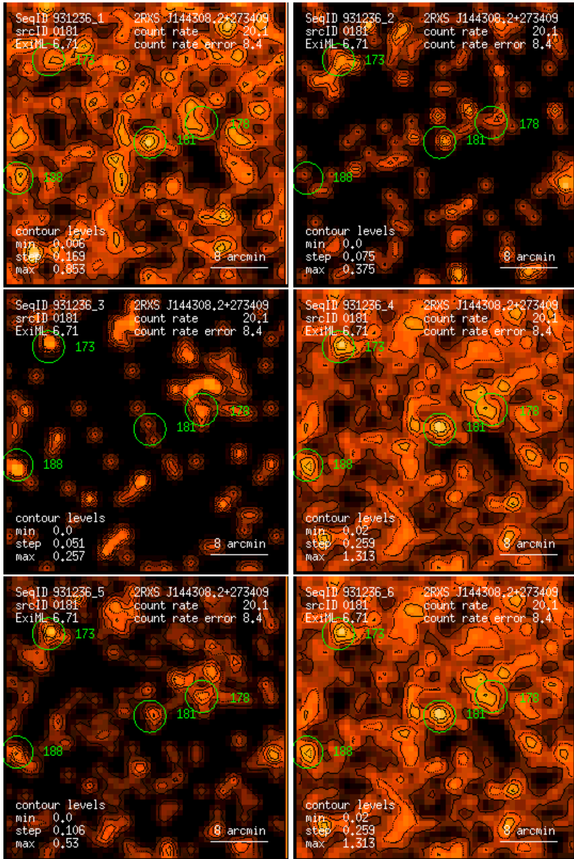
Figure 181: RASS 931236: detection 0181: band rate images, Gaussian filter: (1) PSPC channels 11 – 41, (2) 52 – 90, (3) 91 – 201, (4) 11 – 235, (5) 52 – 201, (6) 11 – 201. Broad band rates in counts/ks. Band rate contour levels in counts/ks/arcmin 2 .
