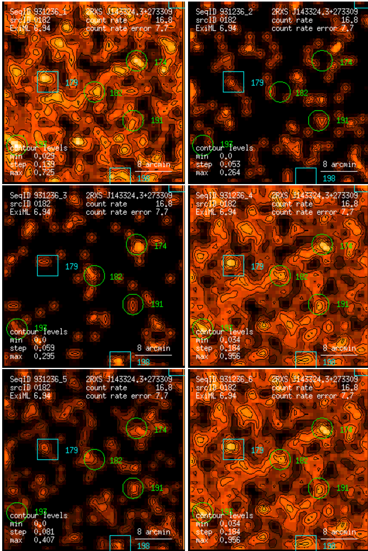
Figure 182: RASS 931236: detection 0182: band rate images, Gaussian filter: (1) PSPC channels 11 – 41, (2) 52 – 90, (3) 91 – 201, (4) 11 – 235, (5) 52 – 201, (6) 11 – 201. Broad band rates in counts/ks. Band rate contour levels in counts/ks/arcmin 2 .
