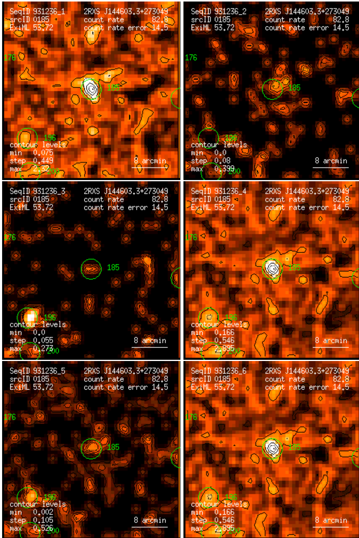
Figure 185: RASS 931236: detection 0185: band rate images, Gaussian filter: (1) PSPC channels 11 – 41, (2) 52 – 90, (3) 91 – 201, (4) 11 – 235, (5) 52 – 201, (6) 11 – 201. Broad band rates in counts/ks. Band rate contour levels in counts/ks/arcmin 2 .
