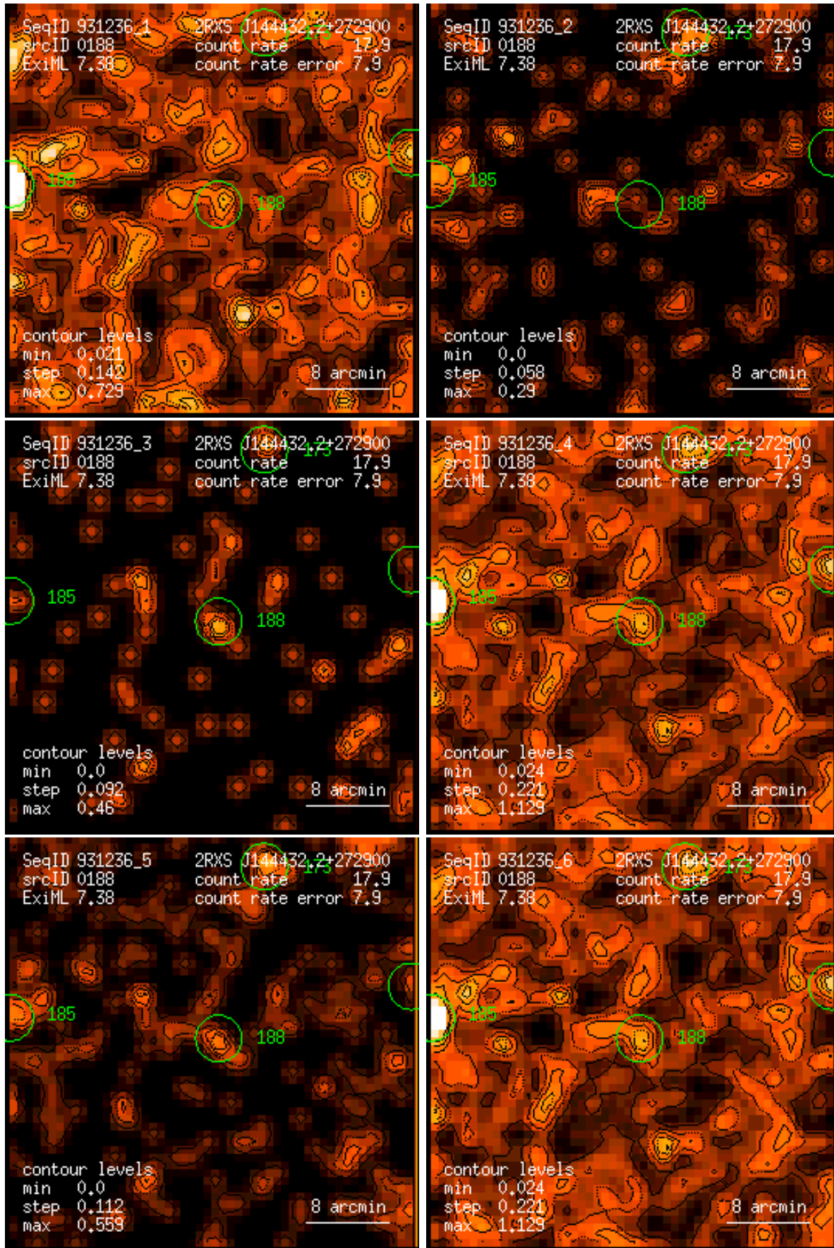
Figure 188: RASS 931236: detection 0188: band rate images, Gaussian filter: (1) PSPC channels 11 – 41, (2) 52 – 90, (3) 91 – 201, (4) 11 – 235, (5) 52 – 201, (6) 11 – 201. Broad band rates in counts/ks. Band rate contour levels in counts/ks/arcmin 2 .
