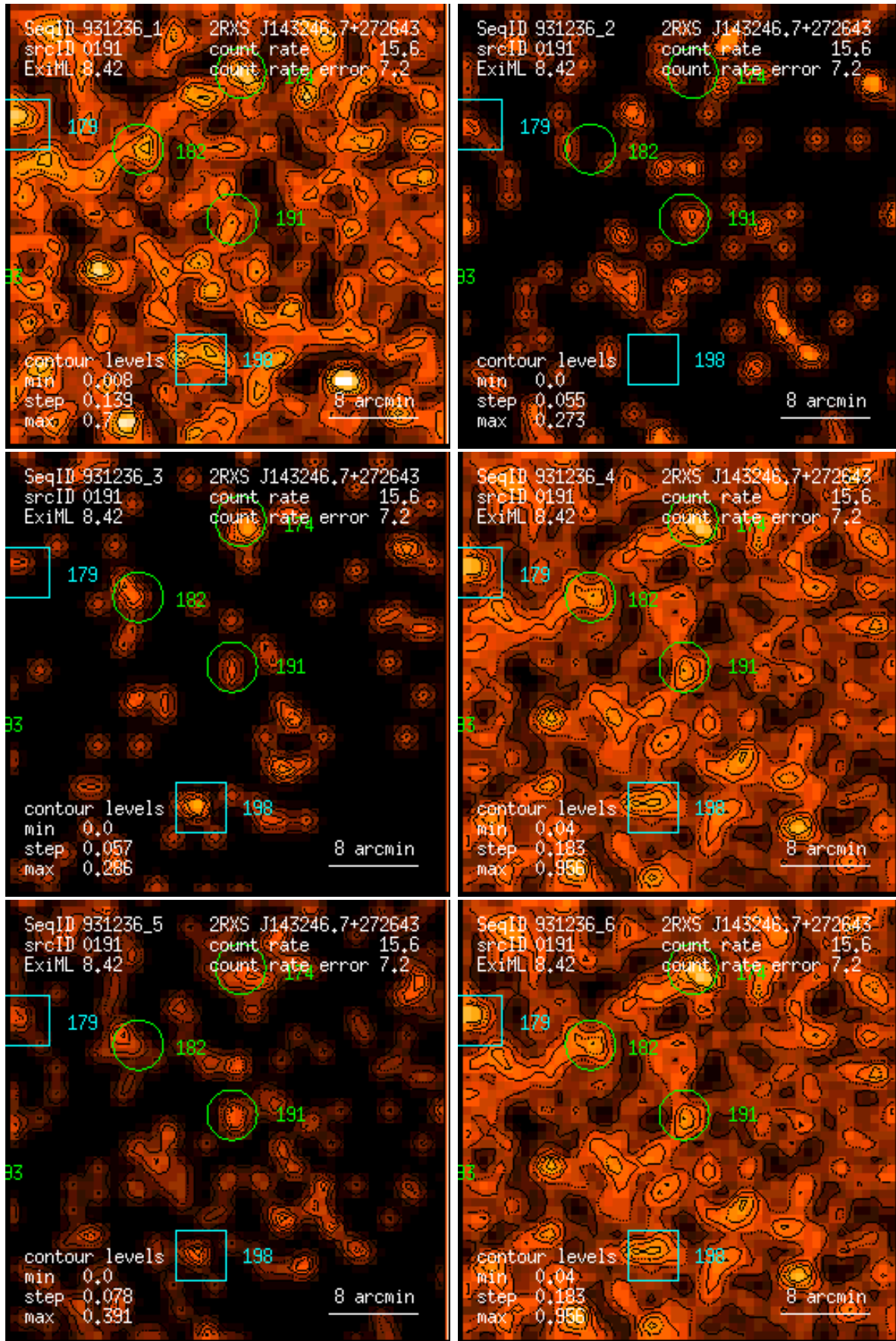
Figure 191: RASS 931236: detection 0191: band rate images, Gaussian filter: (1) PSPC channels 11 – 41, (2) 52 – 90, (3) 91 – 201, (4) 11 – 235, (5) 52 – 201, (6) 11 – 201. Broad band rates in counts/ks. Band rate contour levels in counts/ks/arcmin 2 .
