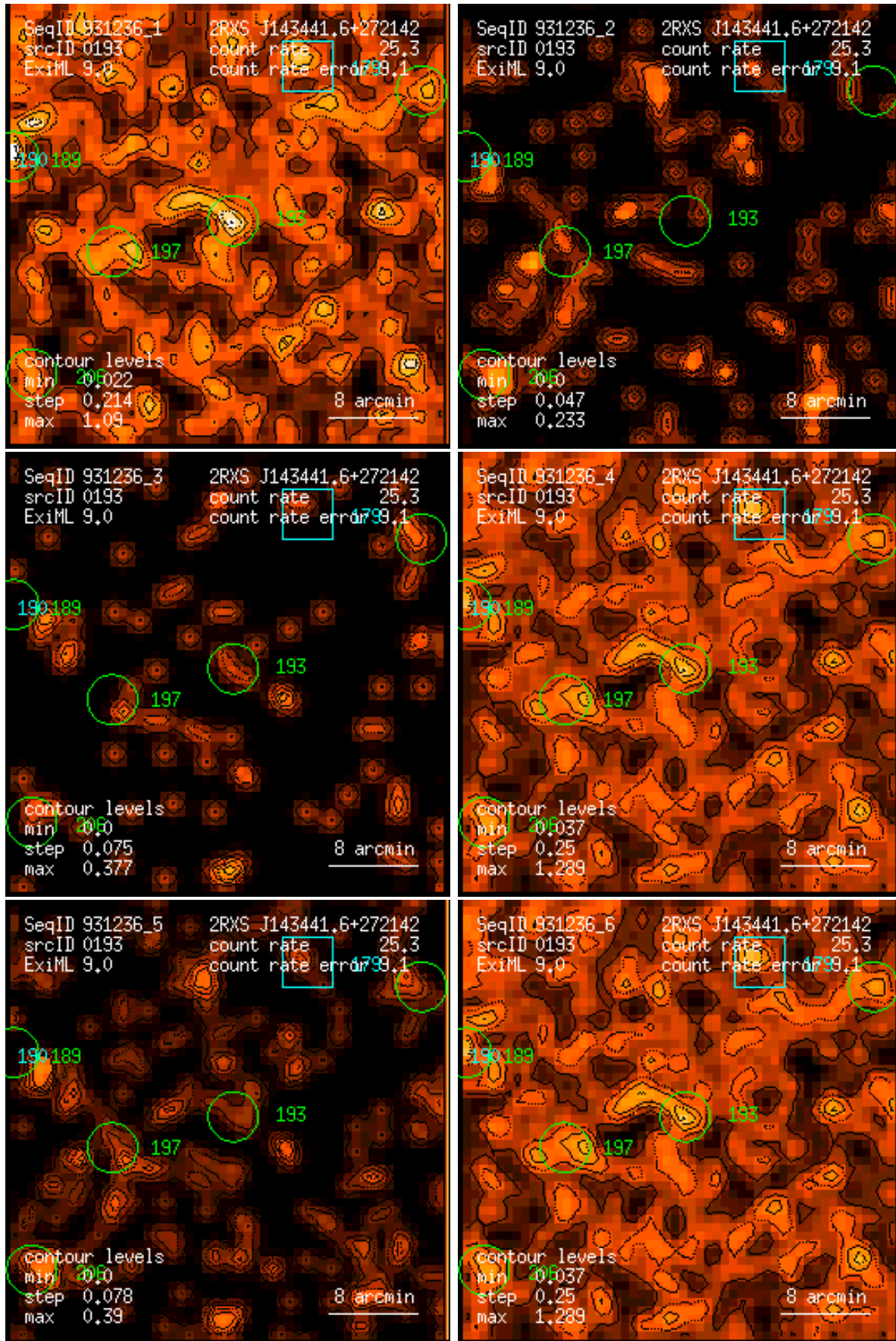
Figure 193: RASS 931236: detection 0193: band rate images, Gaussian filter: (1) PSPC channels 11 – 41, (2) 52 – 90, (3) 91 – 201, (4) 11 – 235, (5) 52 – 201, (6) 11 – 201. Broad band rates in counts/ks. Band rate contour levels in counts/ks/arcmin 2 .
