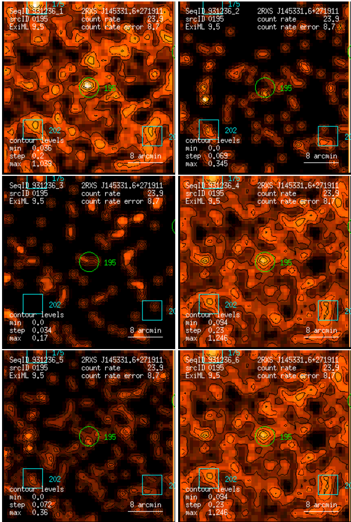
Figure 195: RASS 931236: detection 0195: band rate images, Gaussian filter: (1) PSPC channels 11 – 41, (2) 52 – 90, (3) 91 – 201, (4) 11 – 235, (5) 52 – 201, (6) 11 – 201. Broad band rates in counts/ks. Band rate contour levels in counts/ks/arcmin 2 .
