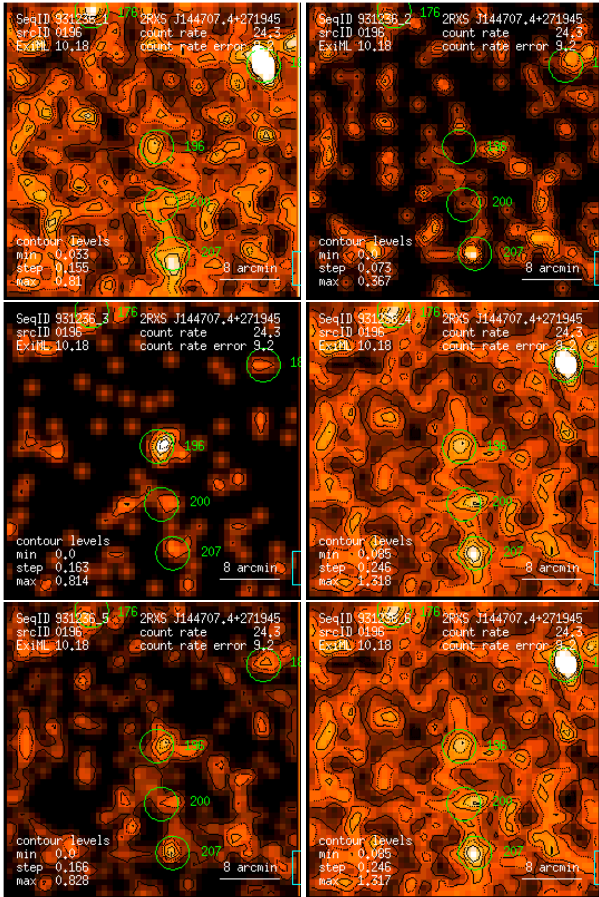
Figure 196: RASS 931236: detection 0196: band rate images, Gaussian filter: (1) PSPC channels 11 – 41, (2) 52 – 90, (3) 91 – 201, (4) 11 – 235, (5) 52 – 201, (6) 11 – 201. Broad band rates in counts/ks. Band rate contour levels in counts/ks/arcmin 2 .
