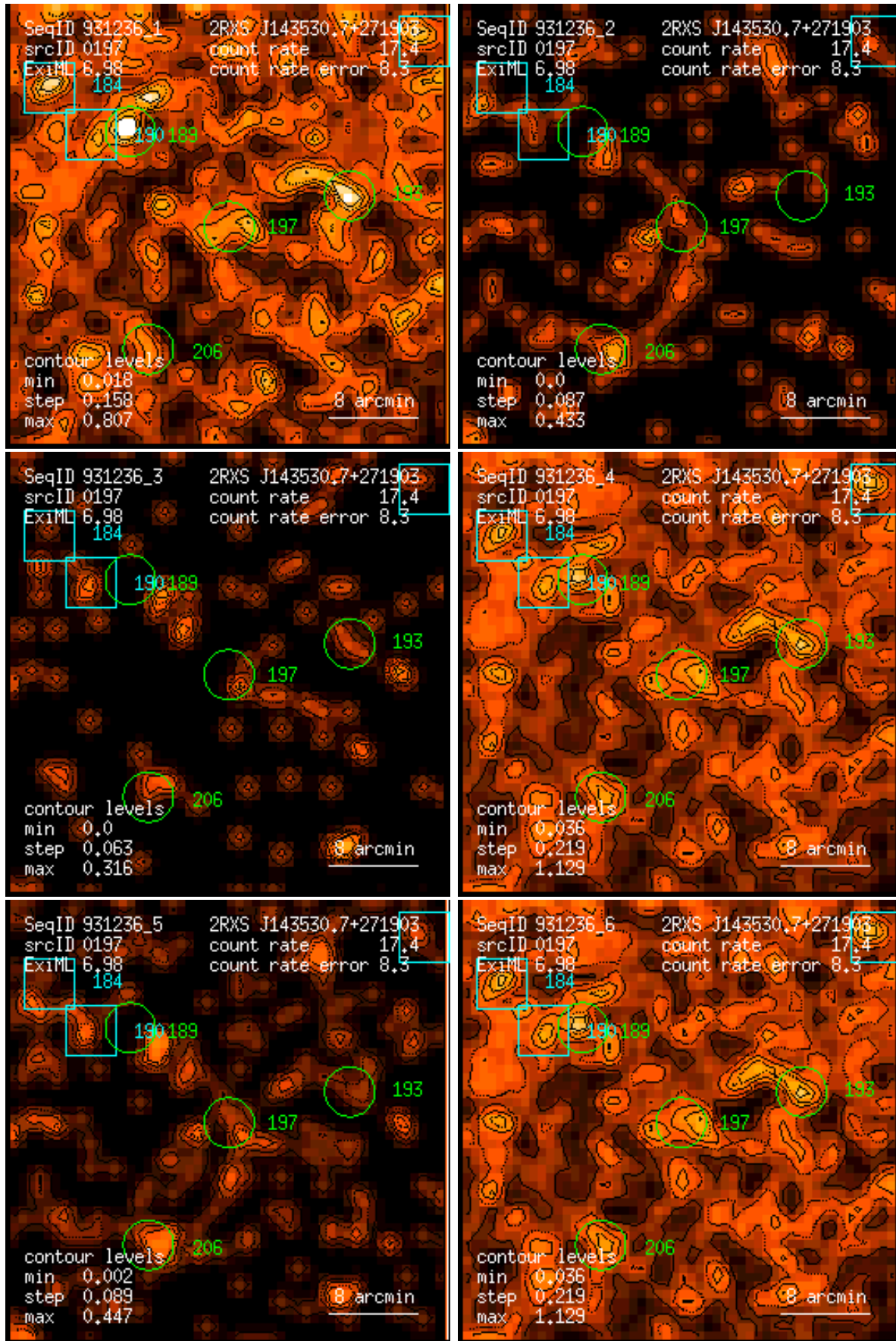
Figure 197: RASS 931236: detection 0197: band rate images, Gaussian filter: (1) PSPC channels 11 – 41, (2) 52 – 90, (3) 91 – 201, (4) 11 – 235, (5) 52 – 201, (6) 11 – 201. Broad band rates in counts/ks. Band rate contour levels in counts/ks/arcmin 2 .
