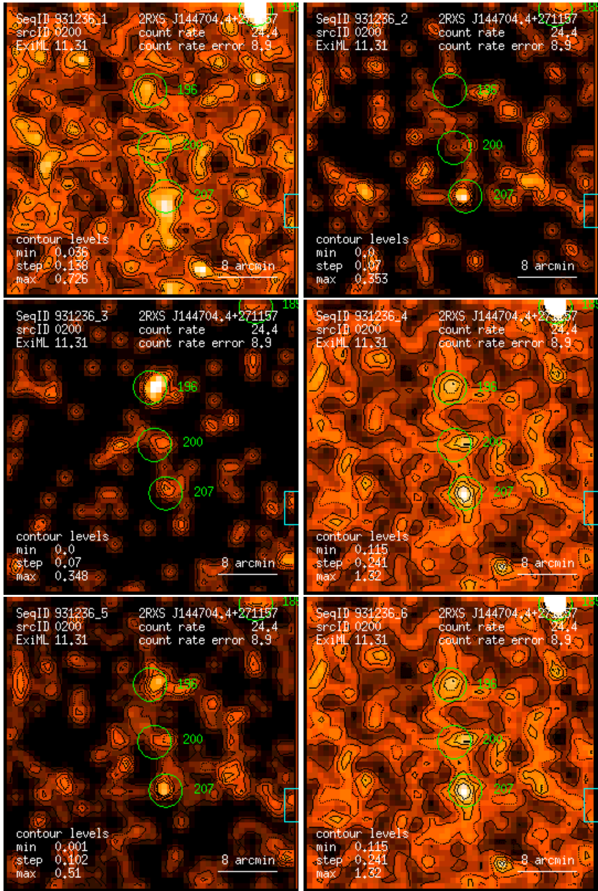
Figure 200: RASS 931236: detection 0200: band rate images, Gaussian filter: (1) PSPC channels 11 – 41, (2) 52 – 90, (3) 91 – 201, (4) 11 – 235, (5) 52 – 201, (6) 11 – 201. Broad band rates in counts/ks. Band rate contour levels in counts/ks/arcmin 2 .
