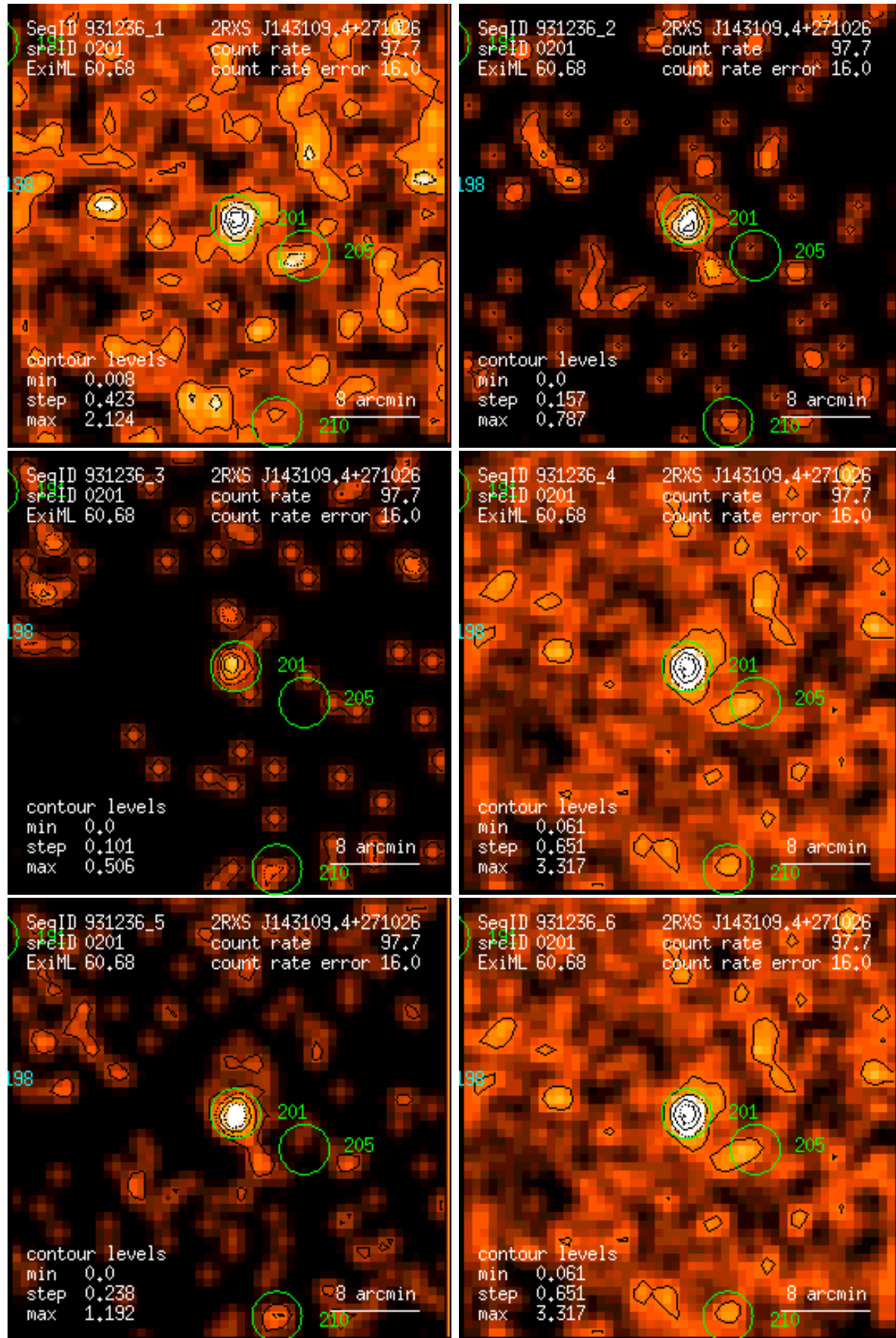
Figure 201: RASS 931236: detection 0201: band rate images, Gaussian filter: (1) PSPC channels 11 – 41, (2) 52 – 90, (3) 91 – 201, (4) 11 – 235, (5) 52 – 201, (6) 11 – 201. Broad band rates in counts/ks. Band rate contour levels in counts/ks/arcmin 2 .
