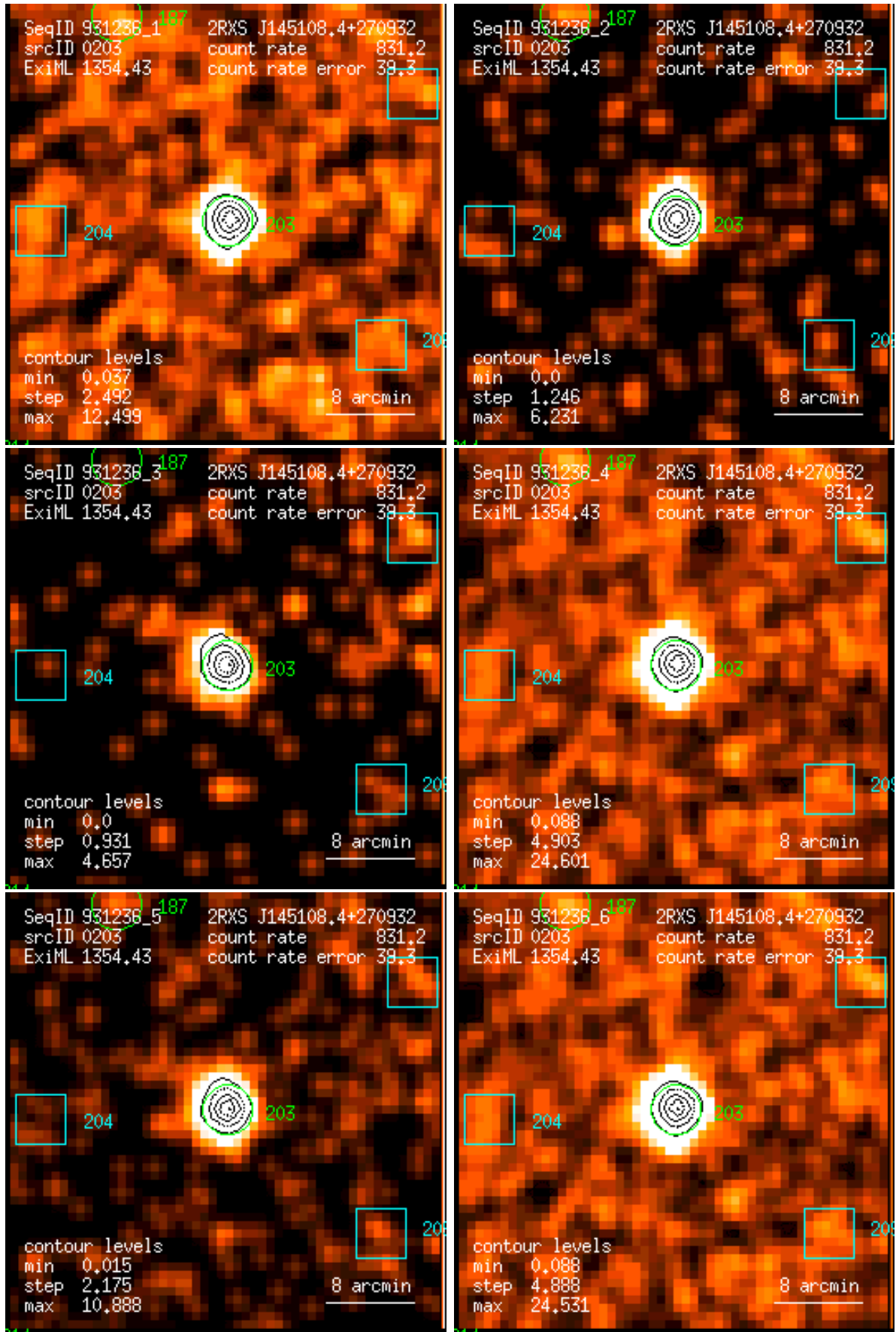
Figure 203: RASS 931236: detection 0203: band rate images, Gaussian filter: (1) PSPC channels 11 – 41, (2) 52 – 90, (3) 91 – 201, (4) 11 – 235, (5) 52 – 201, (6) 11 – 201. Broad band rates in counts/ks. Band rate contour levels in counts/ks/arcmin 2 .
