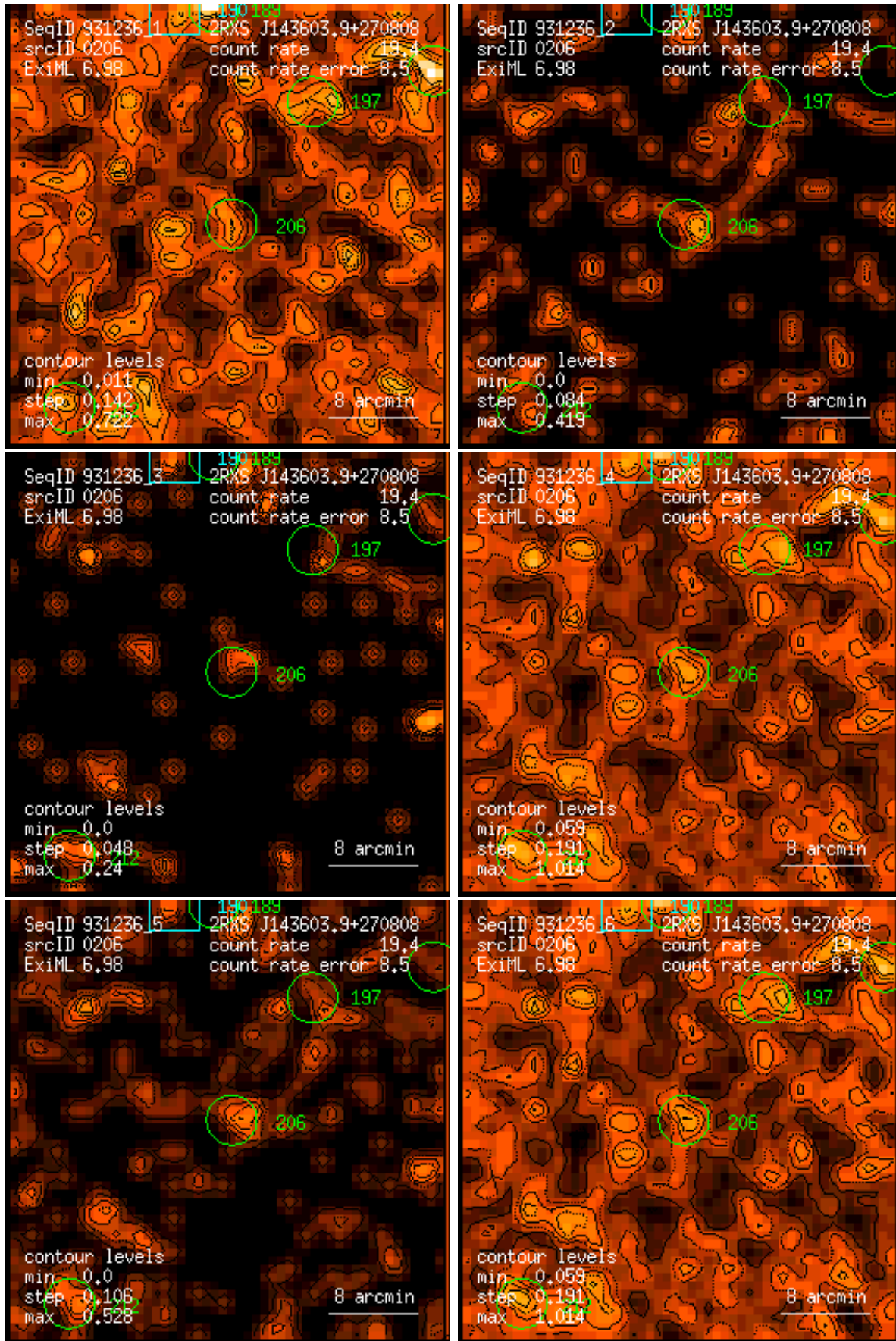
Figure 206: RASS 931236: detection 0206: band rate images, Gaussian filter: (1) PSPC channels 11 – 41, (2) 52 – 90, (3) 91 – 201, (4) 11 – 235, (5) 52 – 201, (6) 11 – 201. Broad band rates in counts/ks. Band rate contour levels in counts/ks/arcmin 2 .
