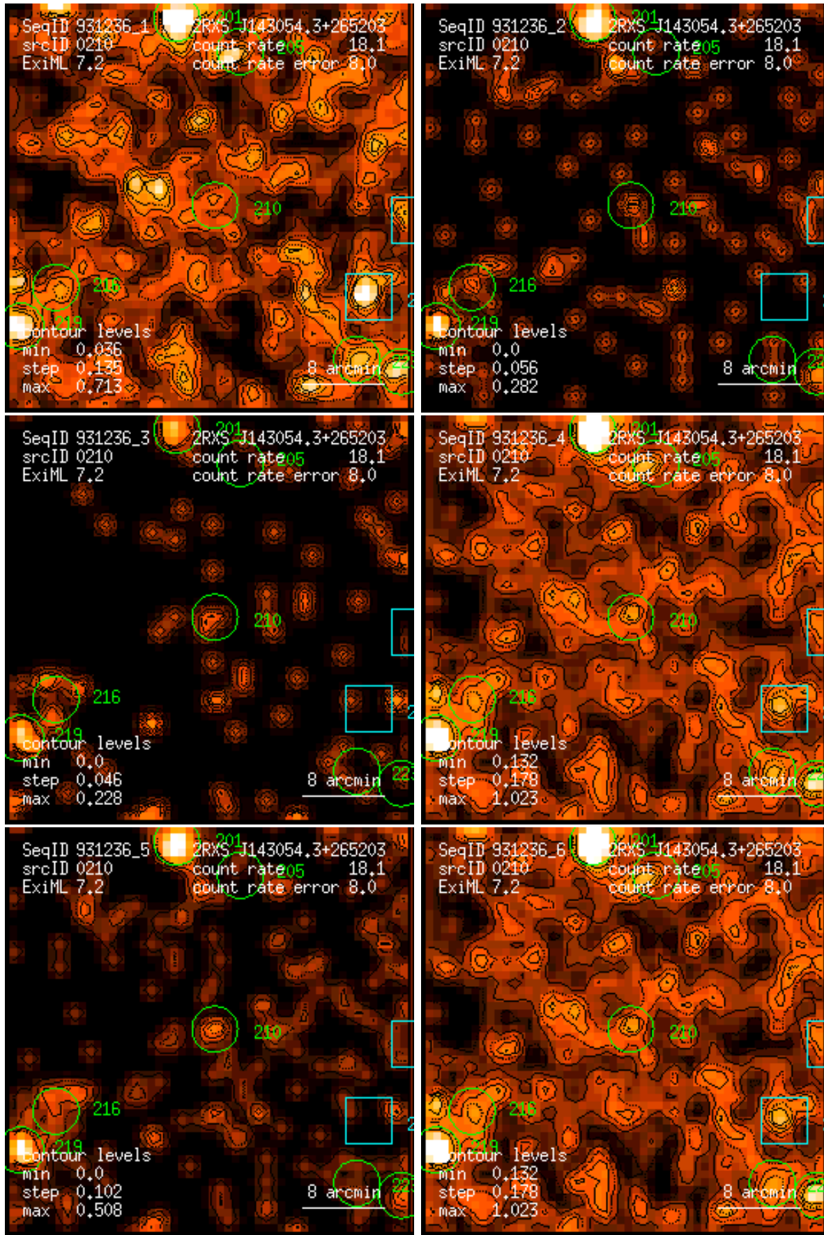
Figure 210: RASS 931236: detection 0210: band rate images, Gaussian filter: (1) PSPC channels 11 – 41, (2) 52 – 90, (3) 91 – 201, (4) 11 – 235, (5) 52 – 201, (6) 11 – 201. Broad band rates in counts/ks. Band rate contour levels in counts/ks/arcmin 2 .
