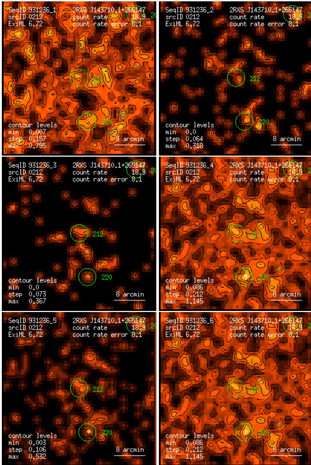
Figure 212: RASS 931236: detection 0212: band rate images, Gaussian filter: (1) PSPC channels 11 – 41, (2) 52 – 90, (3) 91 – 201, (4) 11 – 235, (5) 52 – 201, (6) 11 – 201. Broad band rates in counts/ks. Band rate contour levels in counts/ks/arcmin 2 .
