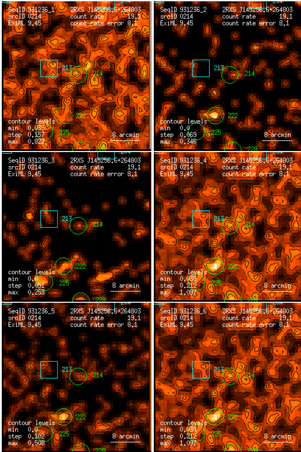
Figure 214: RASS 931236: detection 0214: band rate images, Gaussian filter: (1) PSPC channels 11 – 41, (2) 52 – 90, (3) 91 – 201, (4) 11 – 235, (5) 52 – 201, (6) 11 – 201. Broad band rates in counts/ks. Band rate contour levels in counts/ks/arcmin 2 .
