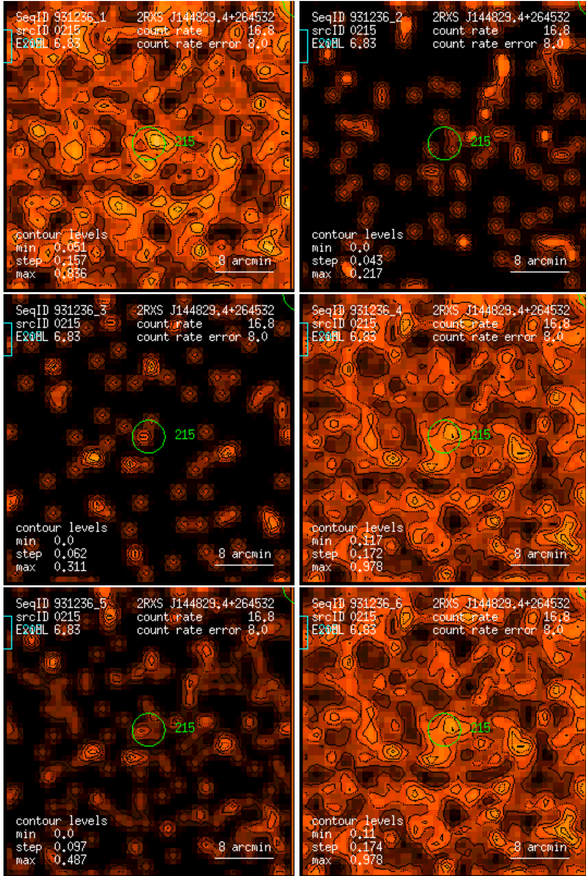
Figure 215: RASS 931236: detection 0215: band rate images, Gaussian filter: (1) PSPC channels 11 – 41, (2) 52 – 90, (3) 91 – 201, (4) 11 – 235, (5) 52 – 201, (6) 11 – 201. Broad band rates in counts/ks. Band rate contour levels in counts/ks/arcmin 2 .
