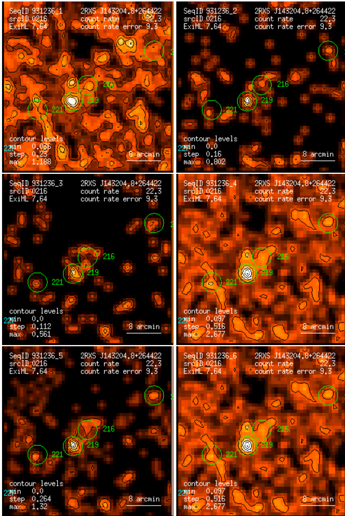
Figure 216: RASS 931236: detection 0216: band rate images, Gaussian filter: (1) PSPC channels 11 – 41, (2) 52 – 90, (3) 91 – 201, (4) 11 – 235, (5) 52 – 201, (6) 11 – 201. Broad band rates in counts/ks. Band rate contour levels in counts/ks/arcmin 2 .
