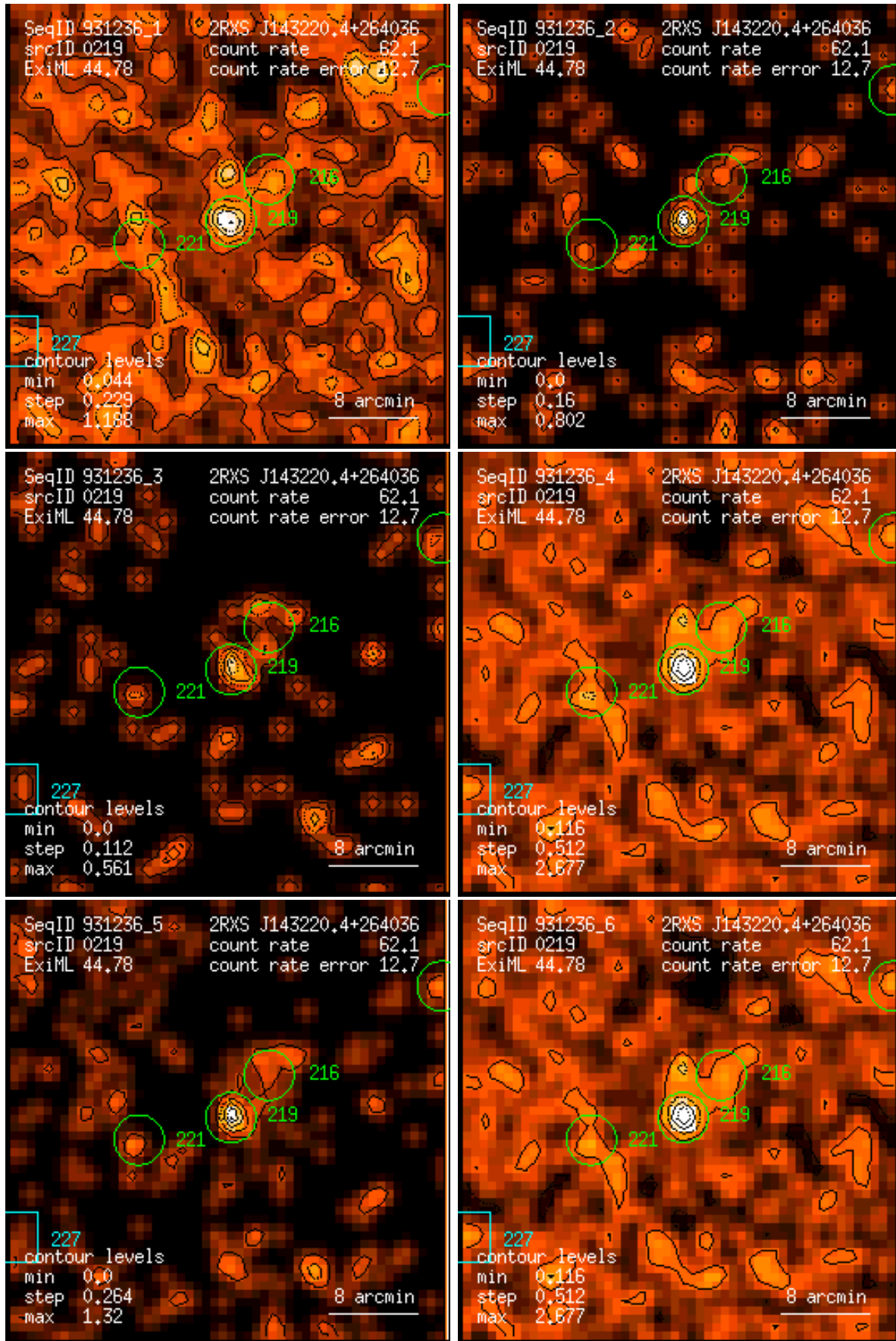
Figure 219: RASS 931236: detection 0219: band rate images, Gaussian filter: (1) PSPC channels 11 – 41, (2) 52 – 90, (3) 91 – 201, (4) 11 – 235, (5) 52 – 201, (6) 11 – 201. Broad band rates in counts/ks. Band rate contour levels in counts/ks/arcmin 2 .
