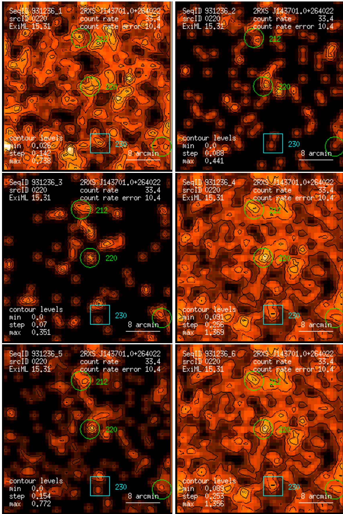
Figure 220: RASS 931236: detection 0220: band rate images, Gaussian filter: (1) PSPC channels 11 – 41, (2) 52 – 90, (3) 91 – 201, (4) 11 – 235, (5) 52 – 201, (6) 11 – 201. Broad band rates in counts/ks. Band rate contour levels in counts/ks/arcmin 2 .
