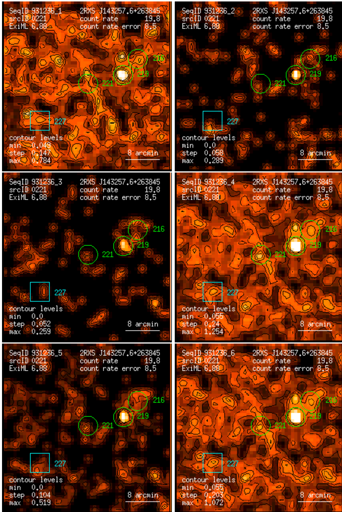
Figure 221: RASS 931236: detection 0221: band rate images, Gaussian filter: (1) PSPC channels 11 – 41, (2) 52 – 90, (3) 91 – 201, (4) 11 – 235, (5) 52 – 201, (6) 11 – 201. Broad band rates in counts/ks. Band rate contour levels in counts/ks/arcmin 2 .
