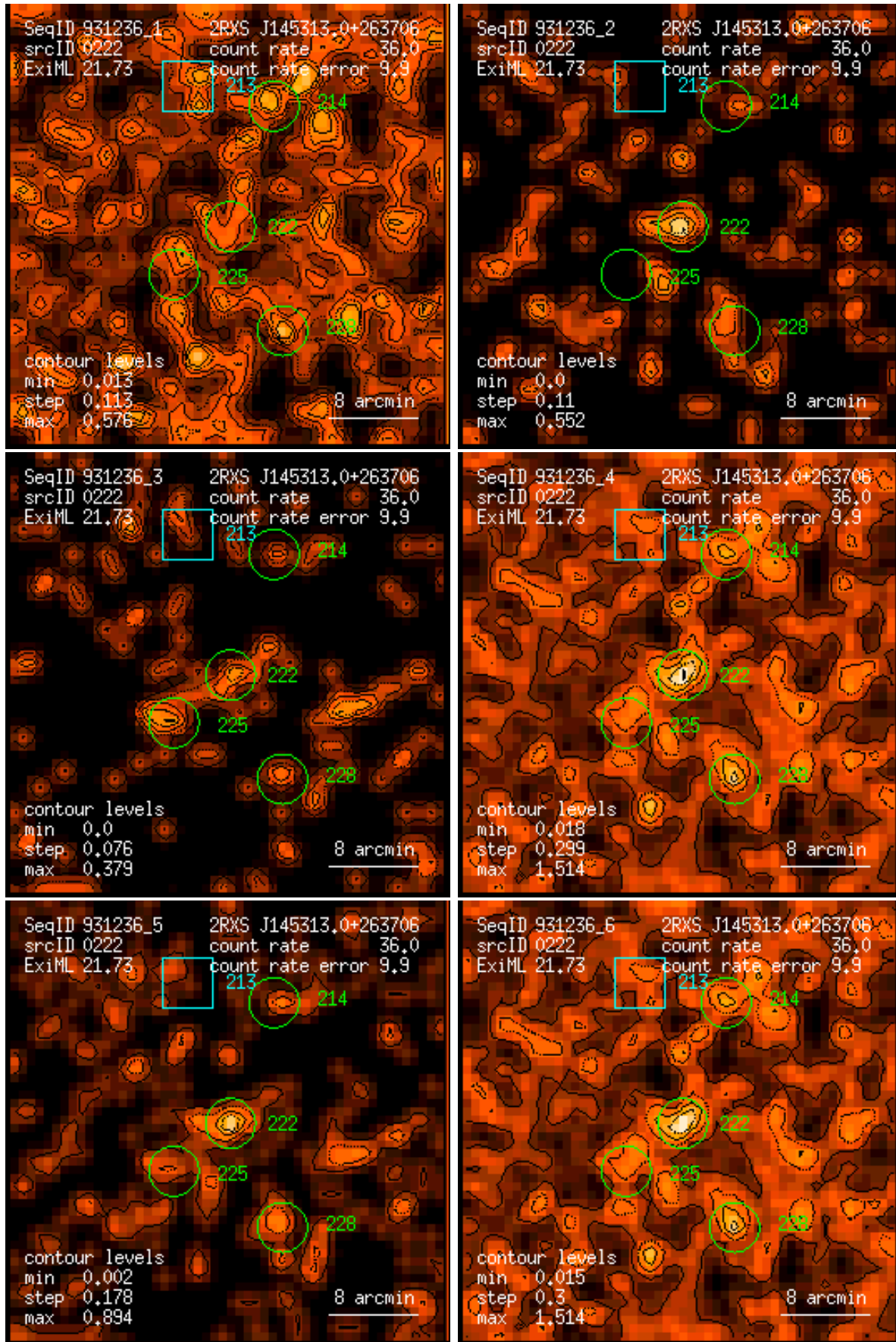
Figure 222: RASS 931236: detection 0222: band rate images, Gaussian filter: (1) PSPC channels 11 – 41, (2) 52 – 90, (3) 91 – 201, (4) 11 – 235, (5) 52 – 201, (6) 11 – 201. Broad band rates in counts/ks. Band rate contour levels in counts/ks/arcmin 2 .
