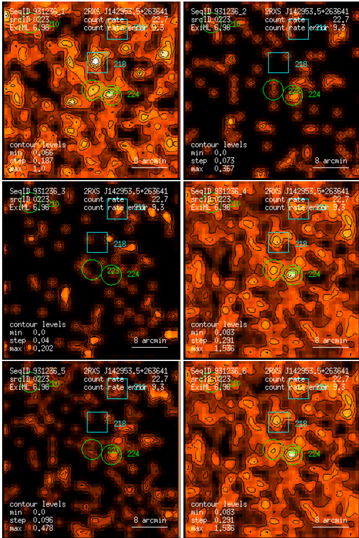
Figure 223: RASS 931236: detection 0223: band rate images, Gaussian filter: (1) PSPC channels 11 – 41, (2) 52 – 90, (3) 91 – 201, (4) 11 – 235, (5) 52 – 201, (6) 11 – 201. Broad band rates in counts/ks. Band rate contour levels in counts/ks/arcmin 2 .
