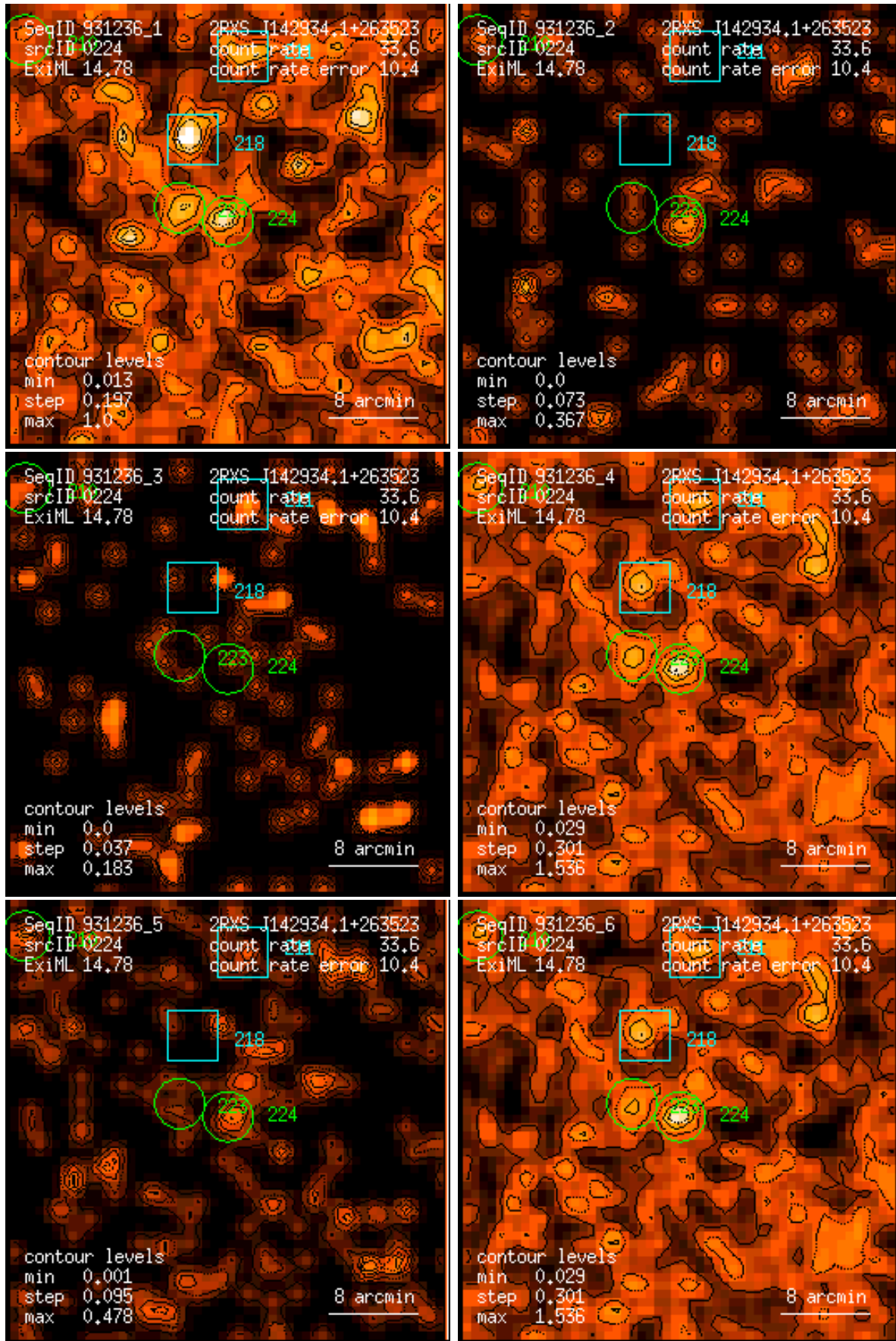
Figure 224: RASS 931236: detection 0224: band rate images, Gaussian filter: (1) PSPC channels 11 – 41, (2) 52 – 90, (3) 91 – 201, (4) 11 – 235, (5) 52 – 201, (6) 11 – 201. Broad band rates in counts/ks. Band rate contour levels in counts/ks/arcmin 2 .
