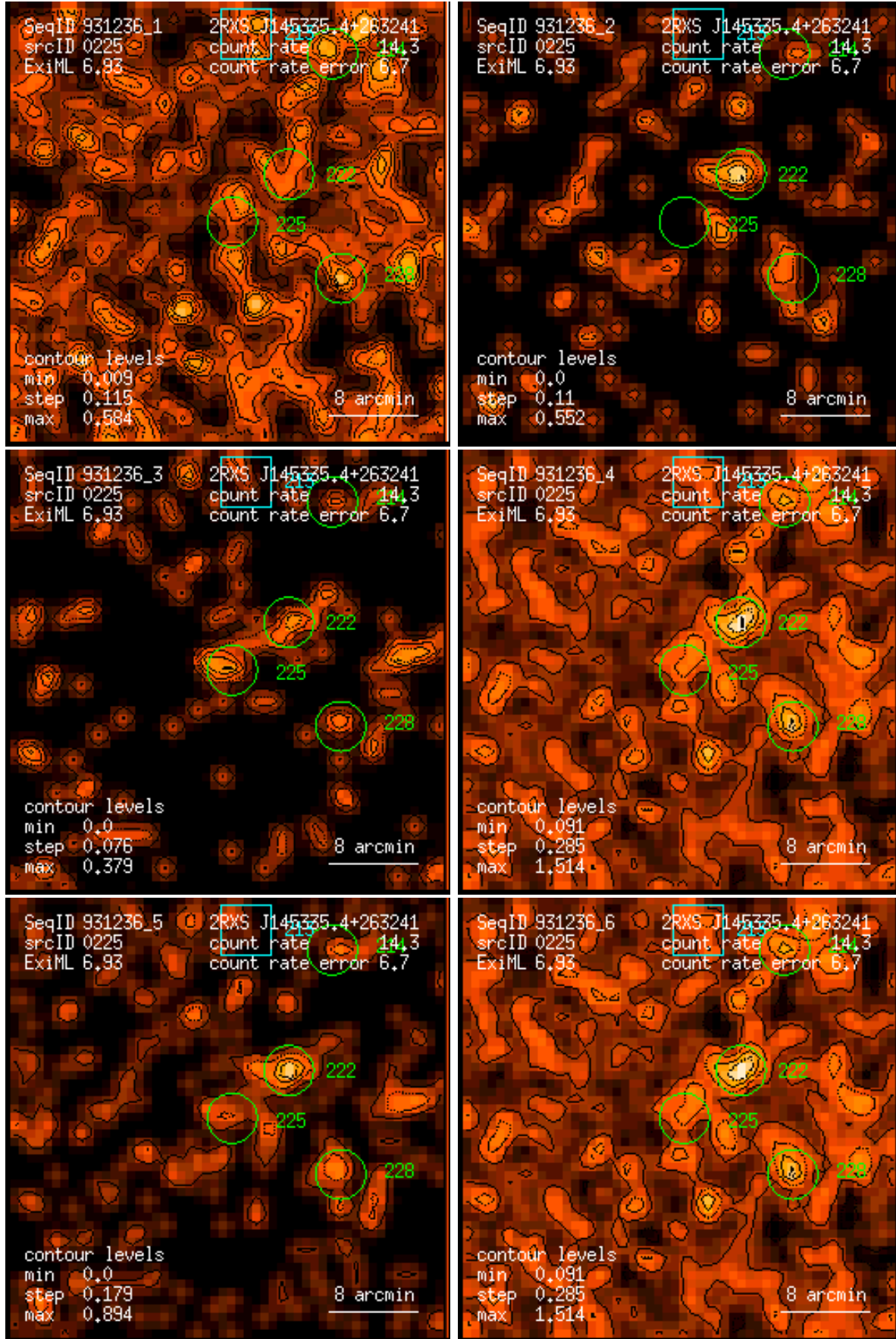
Figure 225: RASS 931236: detection 0225: band rate images, Gaussian filter: (1) PSPC channels 11 – 41, (2) 52 – 90, (3) 91 – 201, (4) 11 – 235, (5) 52 – 201, (6) 11 – 201. Broad band rates in counts/ks. Band rate contour levels in counts/ks/arcmin 2 .
