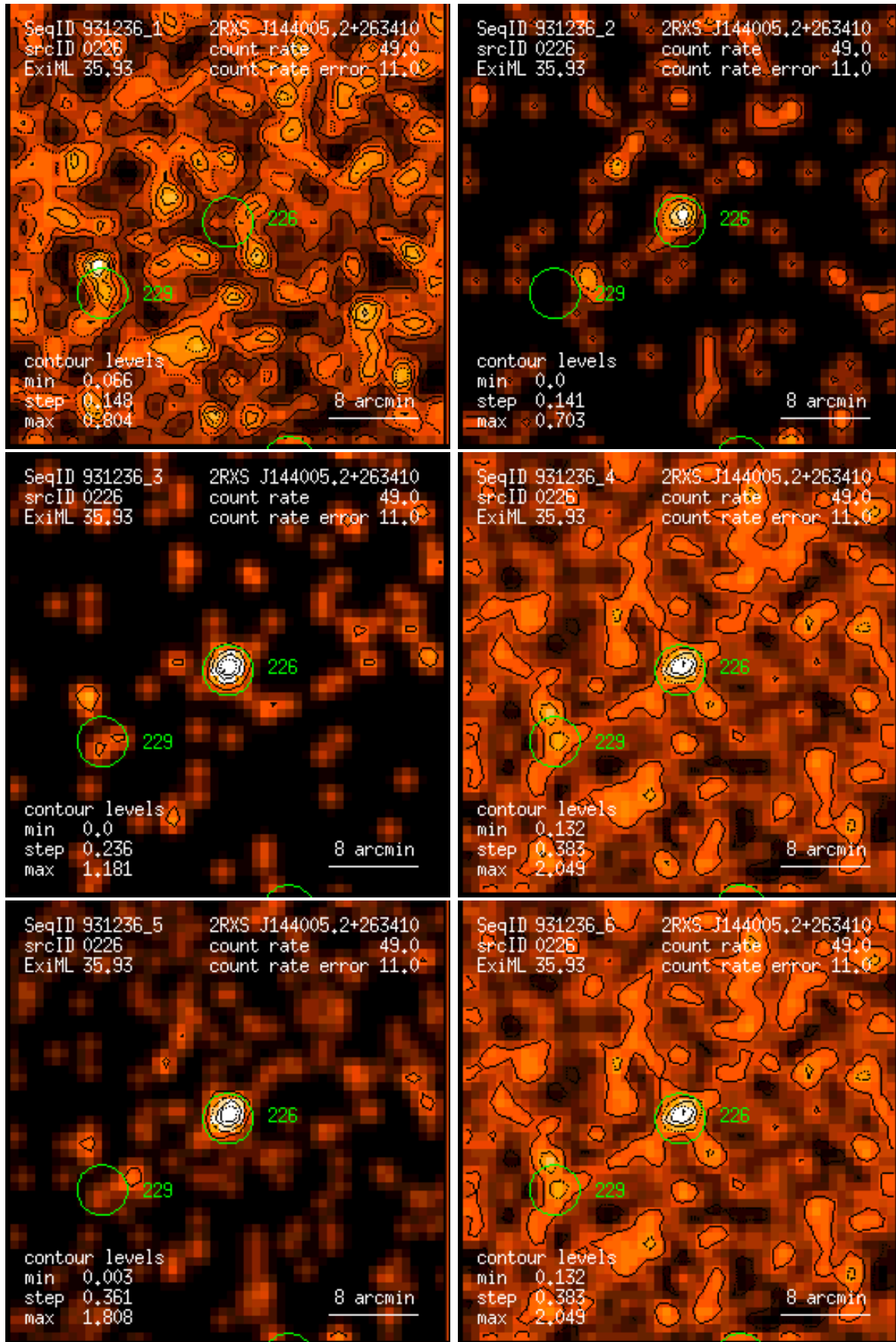
Figure 226: RASS 931236: detection 0226: band rate images, Gaussian filter: (1) PSPC channels 11 – 41, (2) 52 – 90, (3) 91 – 201, (4) 11 – 235, (5) 52 – 201, (6) 11 – 201. Broad band rates in counts/ks. Band rate contour levels in counts/ks/arcmin 2 .
