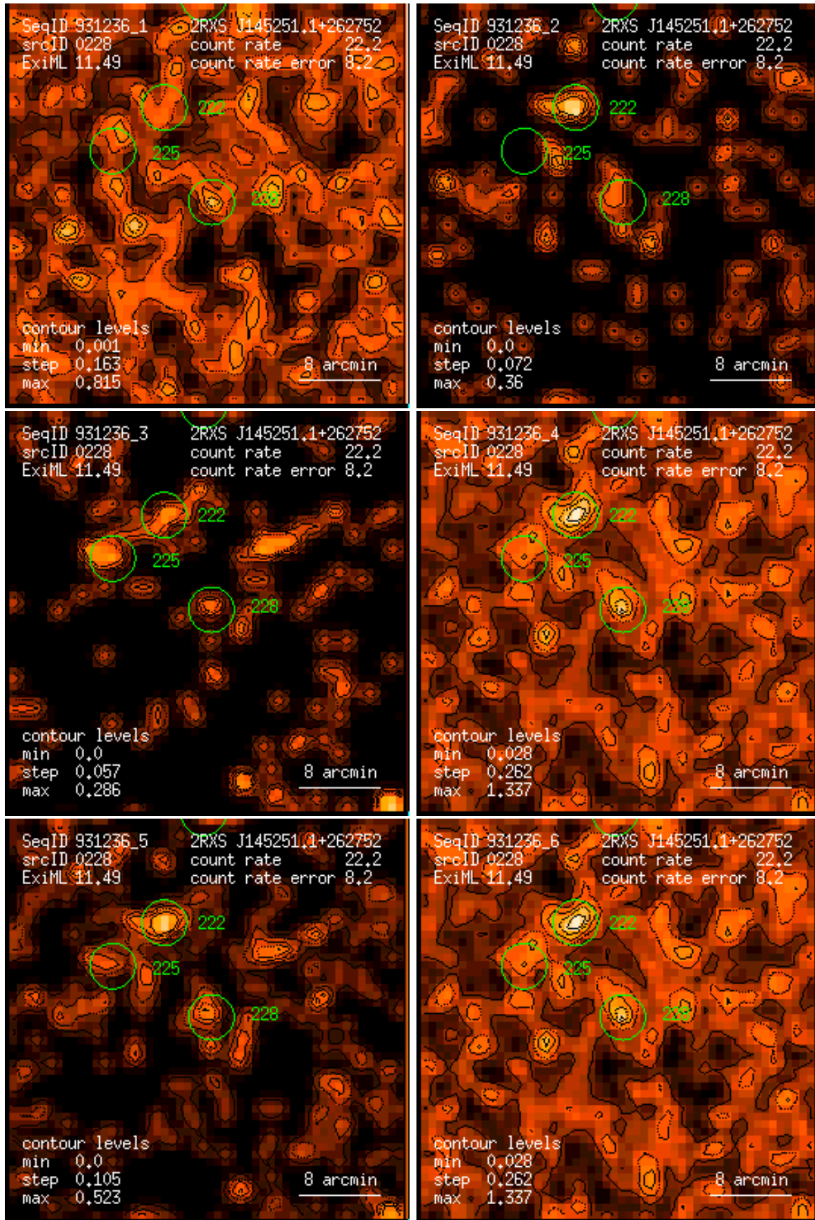
Figure 228: RASS 931236: detection 0228: band rate images, Gaussian filter: (1) PSPC channels 11 – 41, (2) 52 – 90, (3) 91 – 201, (4) 11 – 235, (5) 52 – 201, (6) 11 – 201. Broad band rates in counts/ks. Band rate contour levels in counts/ks/arcmin 2 .
