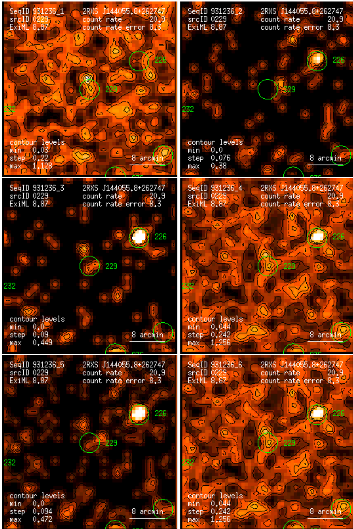
Figure 229: RASS 931236: detection 0229: band rate images, Gaussian filter: (1) PSPC channels 11 – 41, (2) 52 – 90, (3) 91 – 201, (4) 11 – 235, (5) 52 – 201, (6) 11 – 201. Broad band rates in counts/ks. Band rate contour levels in counts/ks/arcmin 2 .
