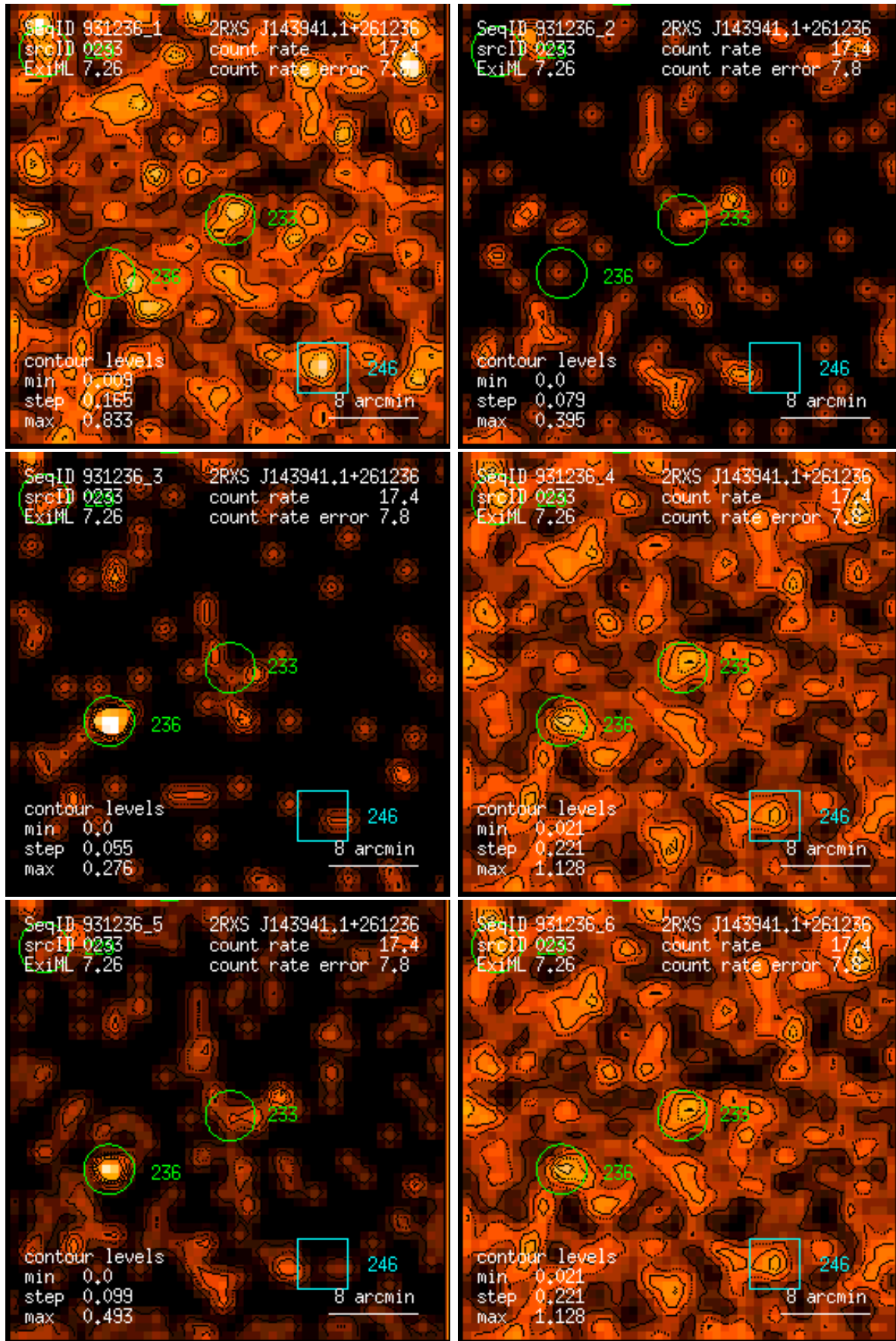
Figure 233: RASS 931236: detection 0233: band rate images, Gaussian filter: (1) PSPC channels 11 – 41, (2) 52 – 90, (3) 91 – 201, (4) 11 – 235, (5) 52 – 201, (6) 11 – 201. Broad band rates in counts/ks. Band rate contour levels in counts/ks/arcmin 2 .
