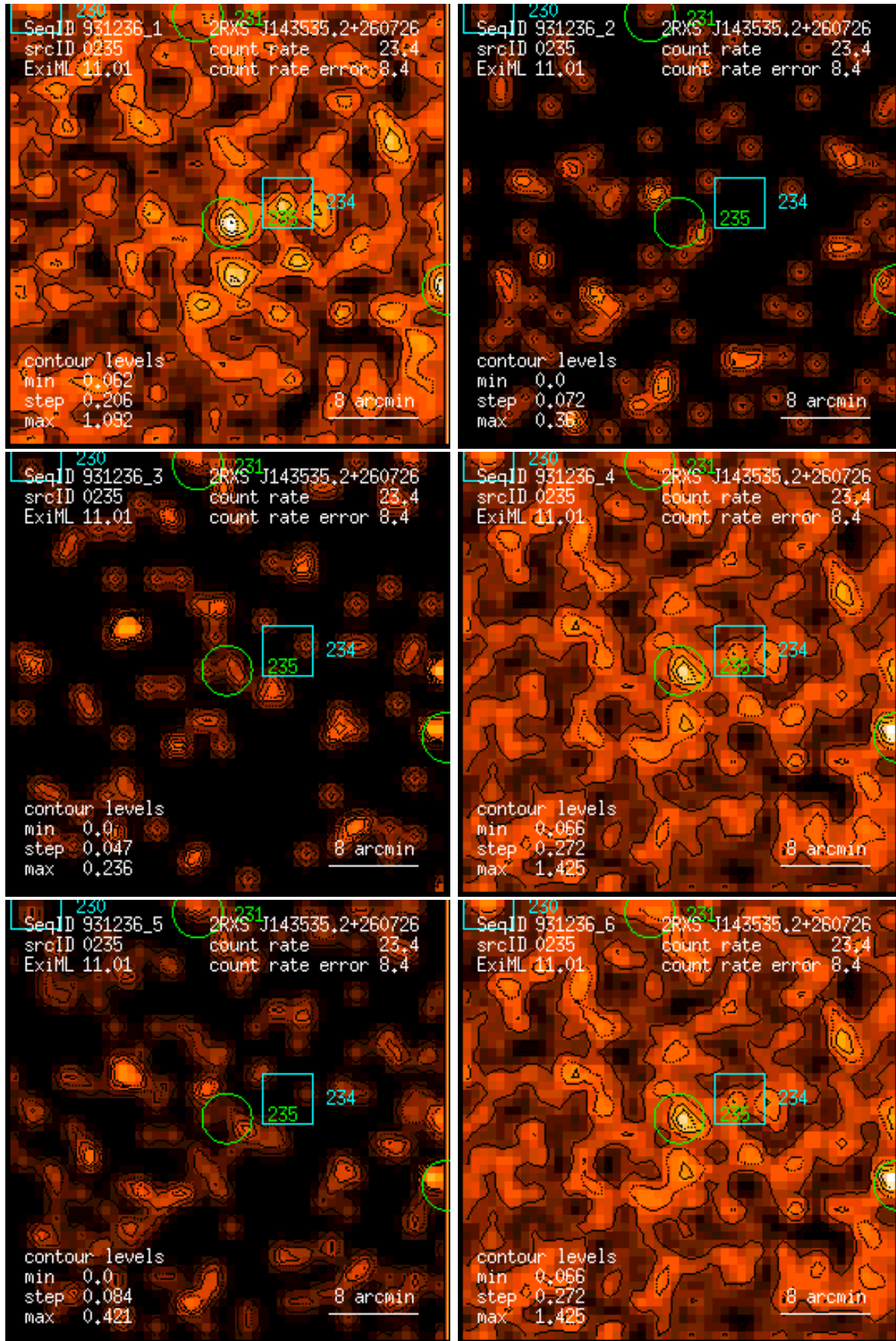
Figure 235: RASS 931236: detection 0235: band rate images, Gaussian filter: (1) PSPC channels 11 – 41, (2) 52 – 90, (3) 91 – 201, (4) 11 – 235, (5) 52 – 201, (6) 11 – 201. Broad band rates in counts/ks. Band rate contour levels in counts/ks/arcmin 2 .
