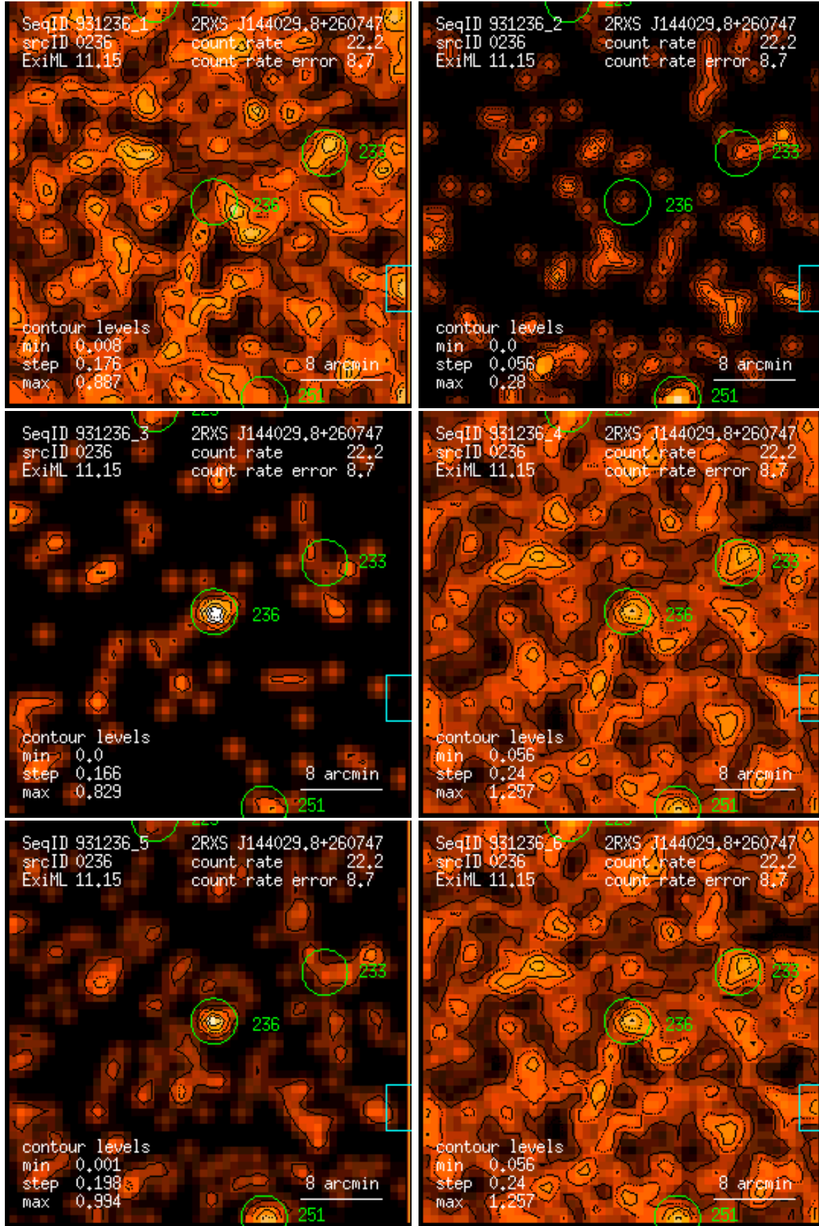
Figure 236: RASS 931236: detection 0236: band rate images, Gaussian filter: (1) PSPC channels 11 – 41, (2) 52 – 90, (3) 91 – 201, (4) 11 – 235, (5) 52 – 201, (6) 11 – 201. Broad band rates in counts/ks. Band rate contour levels in counts/ks/arcmin 2 .
