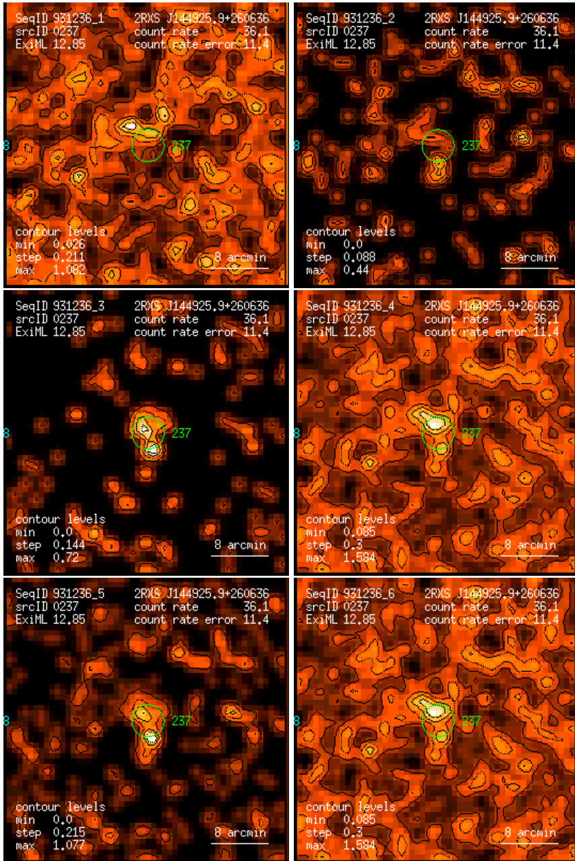
Figure 237: RASS 931236: detection 0237: band rate images, Gaussian filter: (1) PSPC channels 11 – 41, (2) 52 – 90, (3) 91 – 201, (4) 11 – 235, (5) 52 – 201, (6) 11 – 201. Broad band rates in counts/ks. Band rate contour levels in counts/ks/arcmin 2 .
