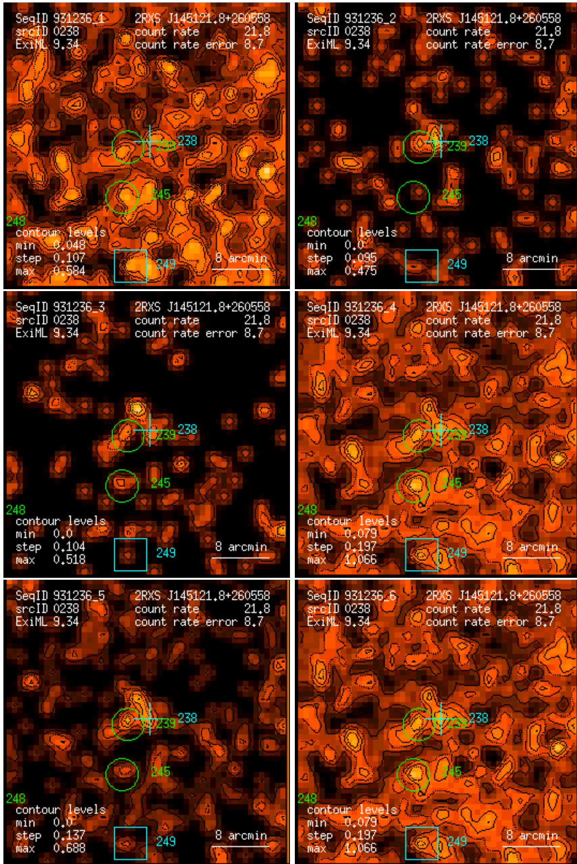
Figure 238: RASS 931236: detection 0238: band rate images, Gaussian filter: (1) PSPC channels 11 – 41, (2) 52 – 90, (3) 91 – 201, (4) 11 – 235, (5) 52 – 201, (6) 11 – 201. Broad band rates in counts/ks. Band rate contour levels in counts/ks/arcmin 2 .
