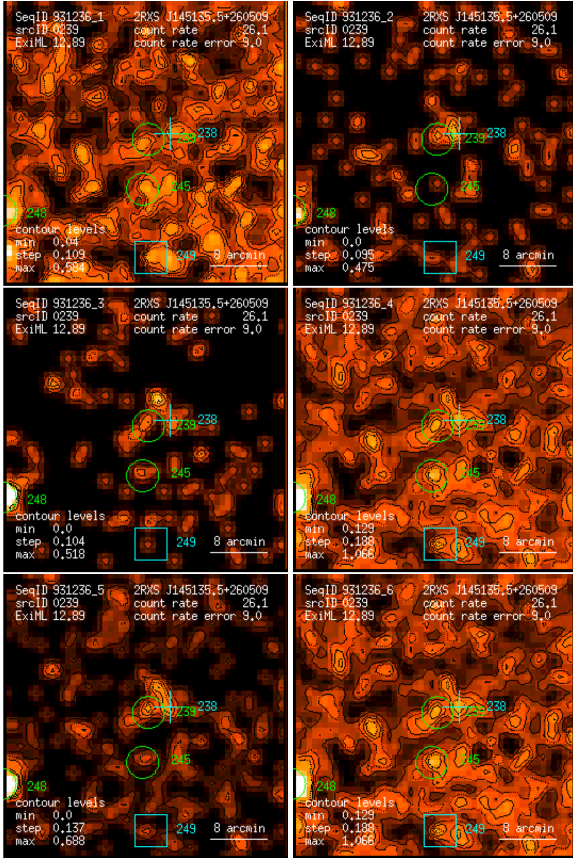
Figure 239: RASS 931236: detection 0239: band rate images, Gaussian filter: (1) PSPC channels 11 – 41, (2) 52 – 90, (3) 91 – 201, (4) 11 – 235, (5) 52 – 201, (6) 11 – 201. Broad band rates in counts/ks. Band rate contour levels in counts/ks/arcmin 2 .
