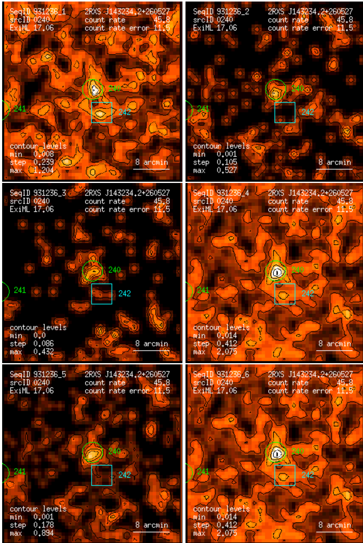
Figure 240: RASS 931236: detection 0240: band rate images, Gaussian filter: (1) PSPC channels 11 – 41, (2) 52 – 90, (3) 91 – 201, (4) 11 – 235, (5) 52 – 201, (6) 11 – 201. Broad band rates in counts/ks. Band rate contour levels in counts/ks/arcmin 2 .
