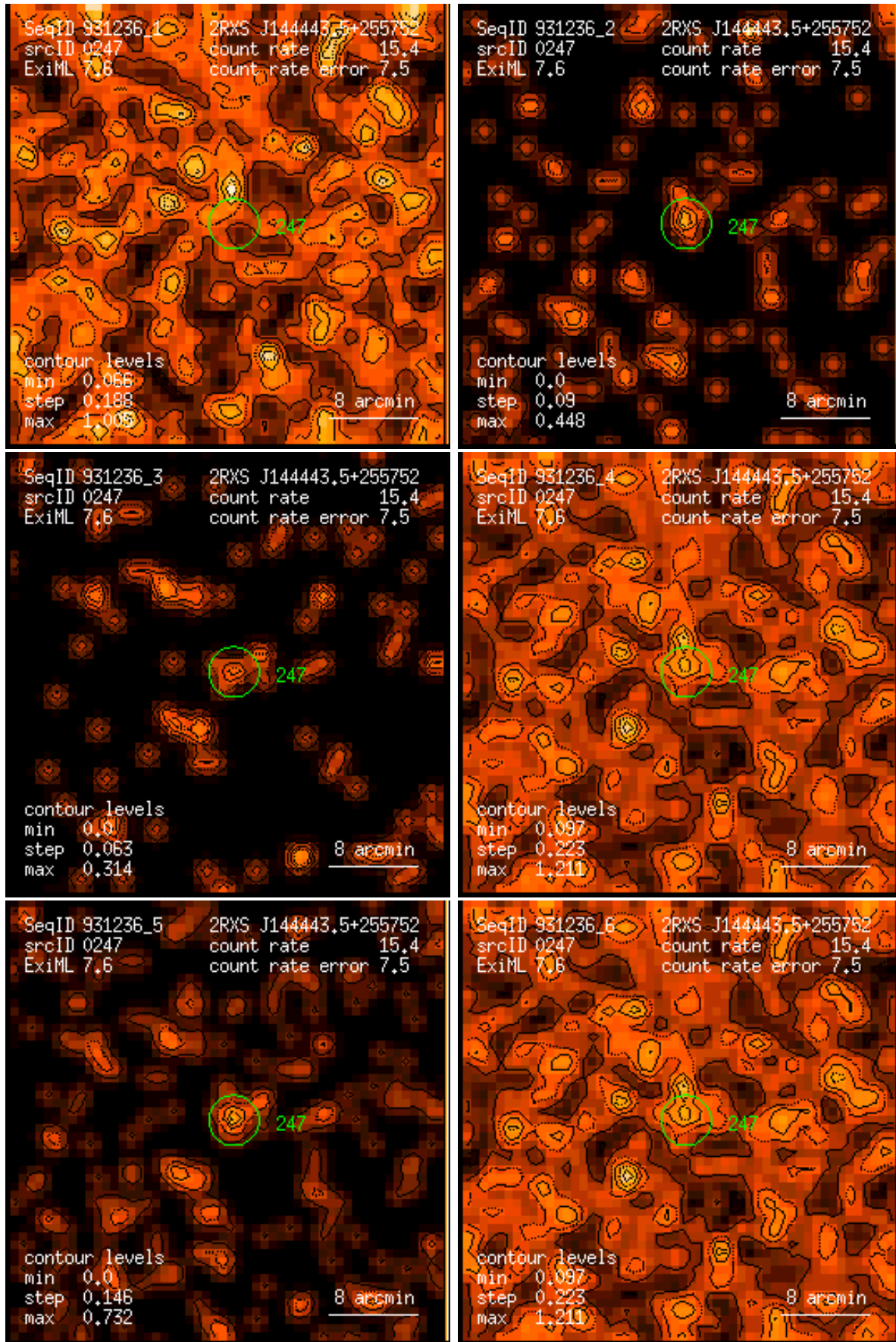
Figure 247: RASS 931236: detection 0247: band rate images, Gaussian filter: (1) PSPC channels 11 – 41, (2) 52 – 90, (3) 91 – 201, (4) 11 – 235, (5) 52 – 201, (6) 11 – 201. Broad band rates in counts/ks. Band rate contour levels in counts/ks/arcmin 2 .
