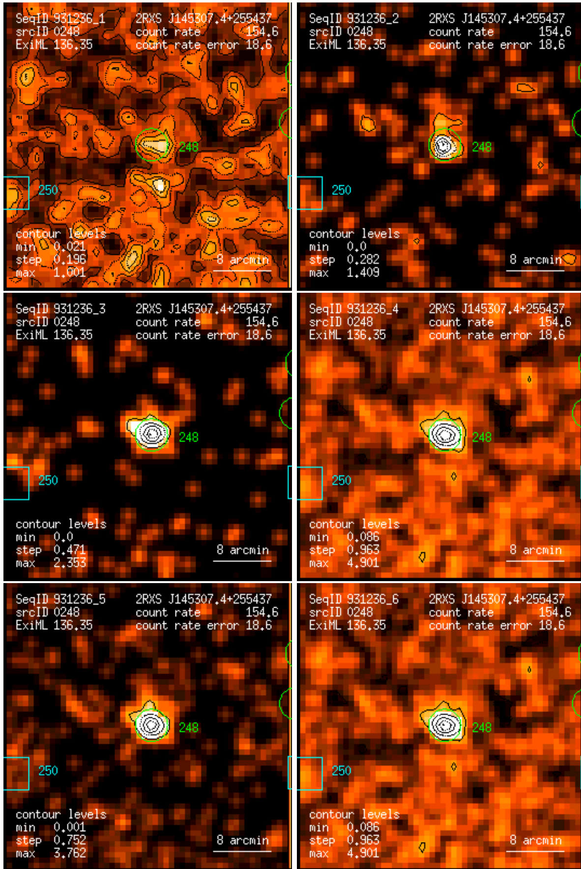
Figure 248: RASS 931236: detection 0248: band rate images, Gaussian filter: (1) PSPC channels 11 – 41, (2) 52 – 90, (3) 91 – 201, (4) 11 – 235, (5) 52 – 201, (6) 11 – 201. Broad band rates in counts/ks. Band rate contour levels in counts/ks/arcmin 2 .
