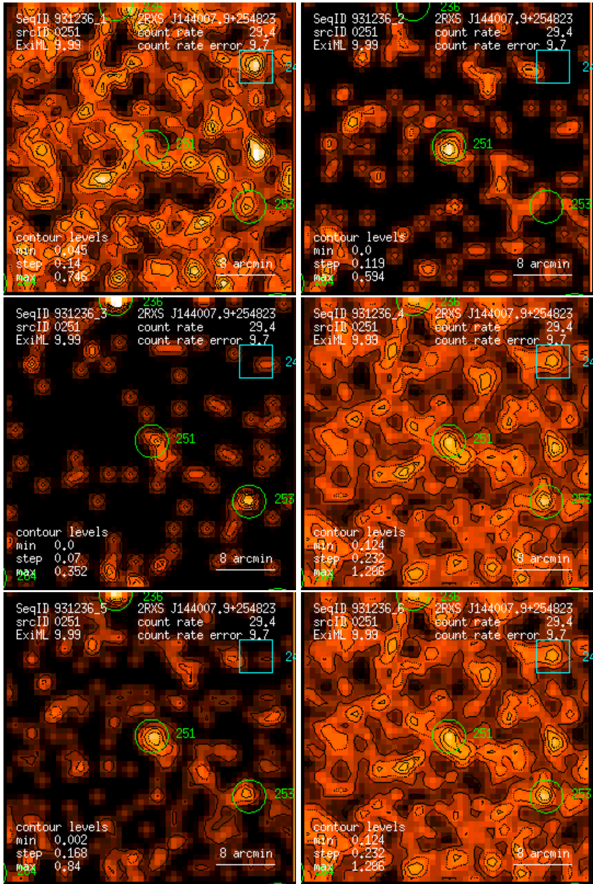
Figure 251: RASS 931236: detection 0251: band rate images, Gaussian filter: (1) PSPC channels 11 – 41, (2) 52 – 90, (3) 91 – 201, (4) 11 – 235, (5) 52 – 201, (6) 11 – 201. Broad band rates in counts/ks. Band rate contour levels in counts/ks/arcmin 2 .
